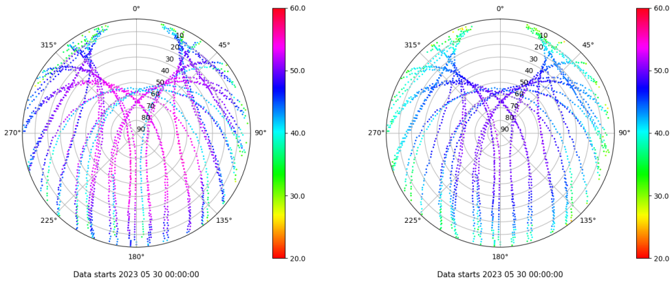
Skyplot for station SINE. Signal to Noise S1C Data file SINE00ESP_R_2023150.xtr Skyplot for station SINE. Signal to Noise S2P Data file SINE00ESP_R_2023150.xtr
