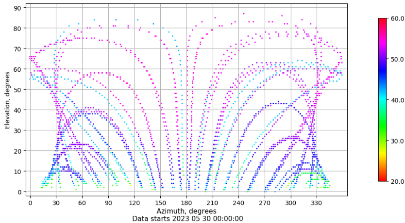
Azimuth-elevation plot for station SINE. Signal to Noise S1C Data file SINE00ESP_R_2023150.xtr
