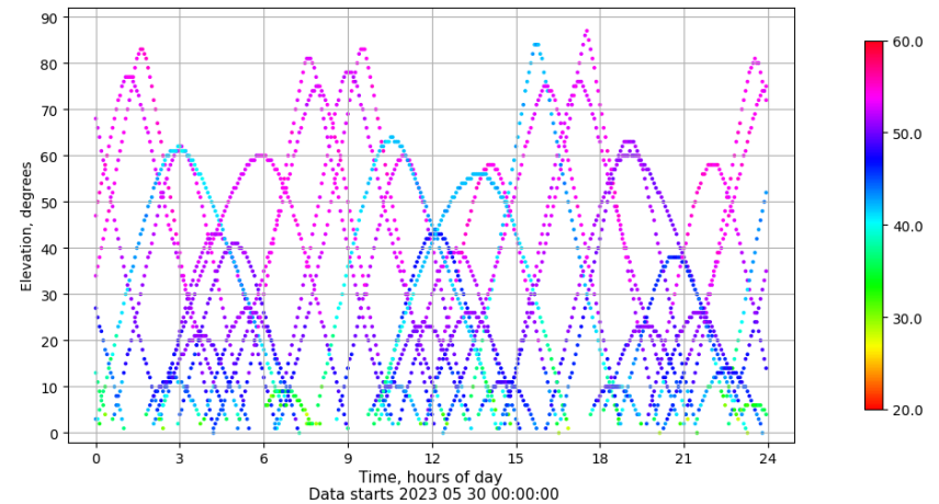
Time-elevation plot for station SINE. Signal to Noise S1C Data file SINE00ESP_R_2023150.xtr
