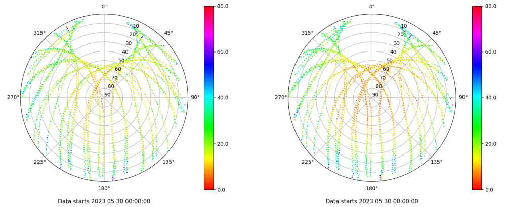
Skyplot for station SINE. Parameter M1C Data file SINE00ESP_R_2023150.xtr Skyplot for station SINE. Parameter M2P Data file SINE00ESP_R_2023150.xtr
