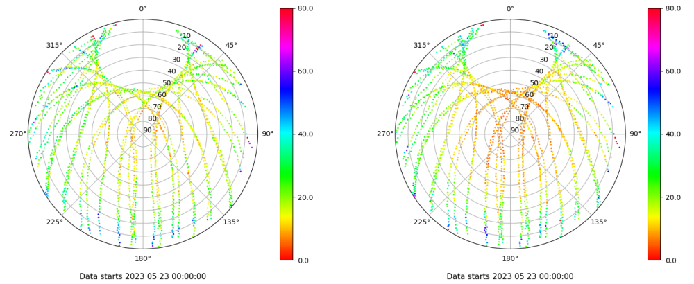
Skyplot for station SINE. Parameter M1C Data file SINE00ESP_R_2023143.xtr Skyplot for station SINE. Parameter M2P Data file SINE00ESP_R_2023143.xtr
