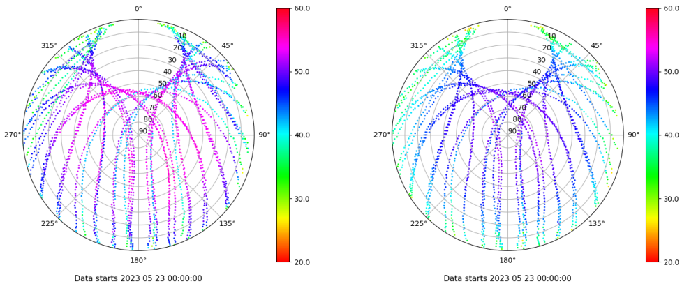
Skyplot for station SINE. Signal to Noise S1C Data file SINE00ESP_R_2023143.xtr Skyplot for station SINE. Signal to Noise S2P Data file SINE00ESP_R_2023143.xtr
