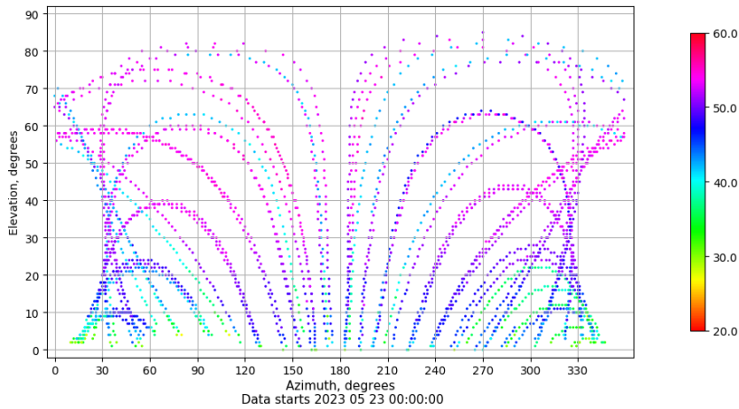
Azimuth-elevation plot for station SINE. Signal to Noise S1C Data file SINE00ESP_R_2023143.xtr
