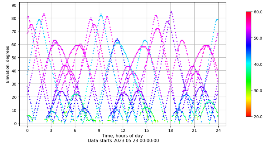
Time-elevation plot for station SINE. Signal to Noise S1C Data file SINE00ESP_R_2023143.xtr
