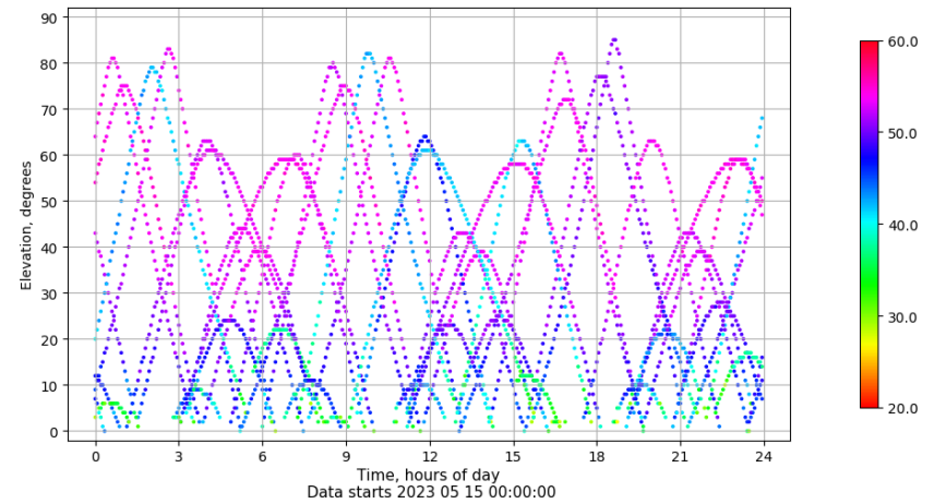
Time-elevation plot for station SINE. Signal to Noise S1C Data file SINE00ESP_R_2023135.xtr
