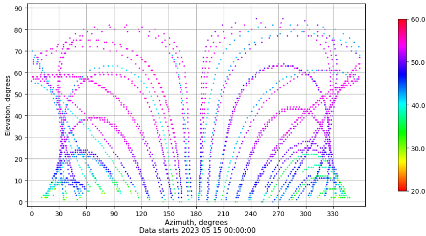
Azimuth-elevation plot for station SINE. Signal to Noise S1C Data file SINE00ESP_R_2023135.xtr
