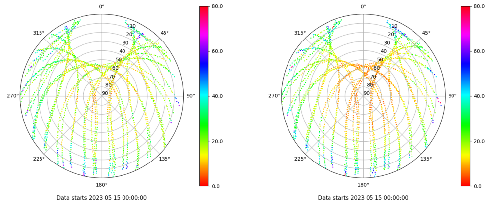
Skyplot for station SINE. Parameter M1C Data file SINE00ESP_R_2023135.xtr Skyplot for station SINE. Parameter M2P Data file SINE00ESP_R_2023135.xtr
