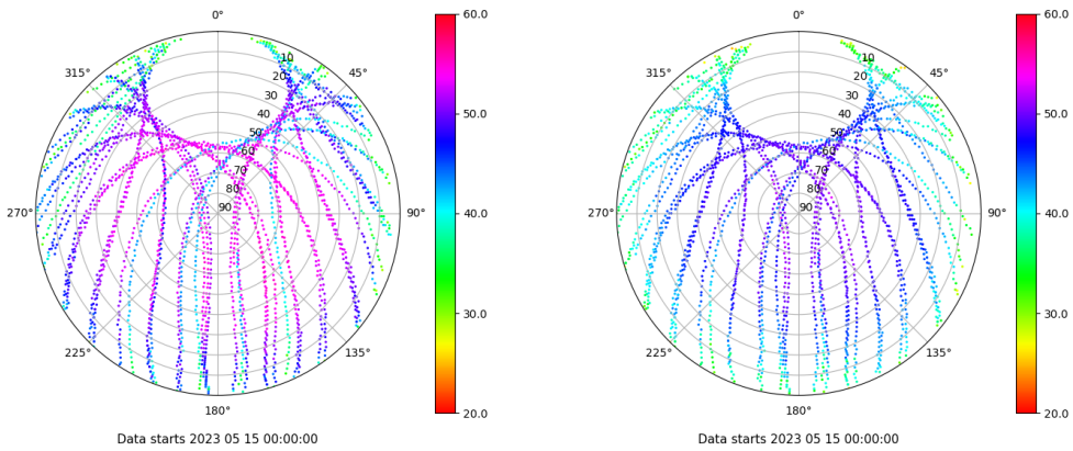
Skyplot for station SINE. Signal to Noise S1C Data file SINE00ESP_R_2023135.xtr Skyplot for station SINE. Signal to Noise S2P Data file SINE00ESP_R_2023135.xtr
