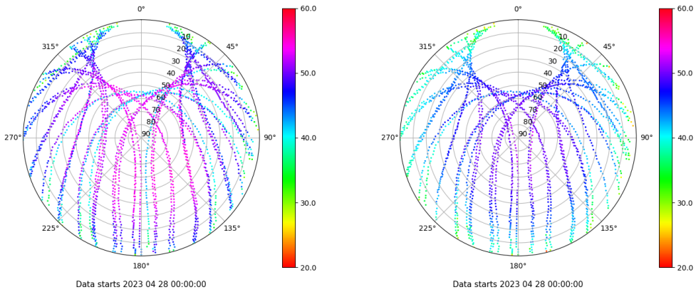
Skyplot for station SINE. Signal to Noise S1C Data file SINE00ESP_R_2023118.xtr Skyplot for station SINE. Signal to Noise S2P Data file SINE00ESP_R_2023118.xtr
