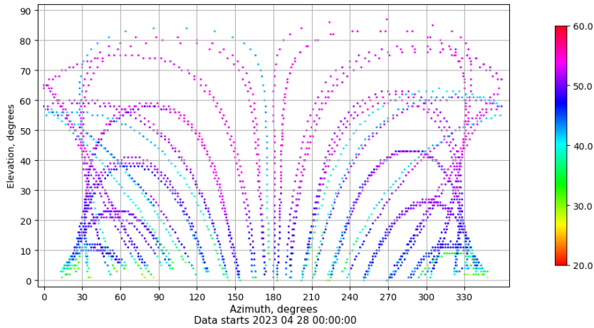
Azimuth-elevation plot for station SINE. Signal to Noise S1C Data file SINE00ESP_R_2023118.xtr
