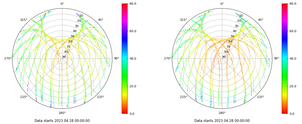
Skyplot for station SINE. Parameter M1C Data file SINE00ESP_R_2023118.xtr Skyplot for station SINE. Parameter M2P Data file SINE00ESP_R_2023118.xtr
