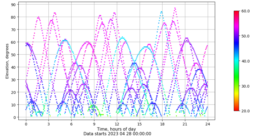
Time-elevation plot for station SINE. Signal to Noise S1C Data file SINE00ESP_R_2023118.xtr
