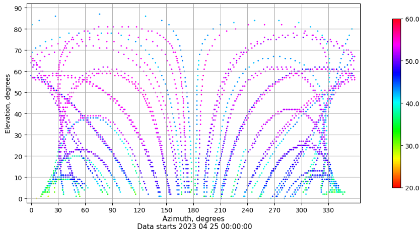
Azimuth-elevation plot for station SINE. Signal to Noise S1C Data file SINE00ESP_R_2023115.xtr
