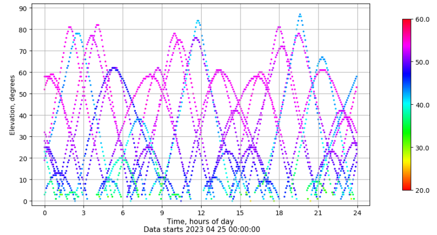
Time-elevation plot for station SINE. Signal to Noise S1C Data file SINE00ESP_R_2023115.xtr
