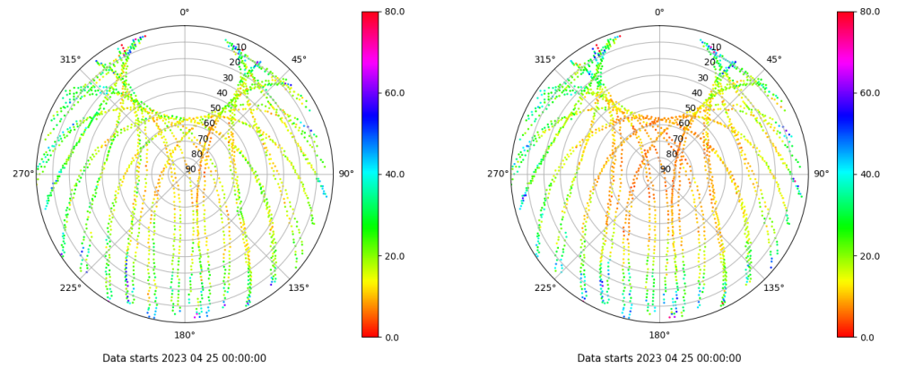
Skyplot for station SINE. Parameter M1C Data file SINE00ESP_R_2023115.xtr Skyplot for station SINE. Parameter M2P Data file SINE00ESP_R_2023115.xtr
