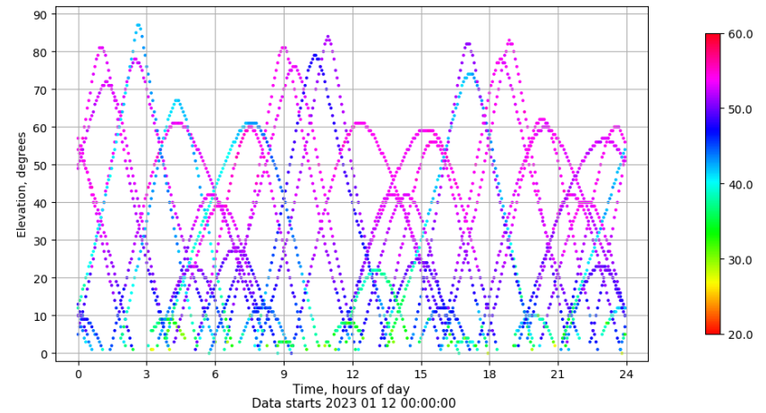
Time-elevation plot for station SINE. Signal to Noise S1C Data file SINE00ESP_R_2023012.xtr
