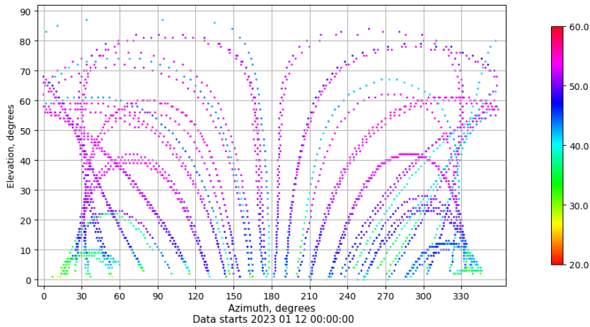
Azimuth-elevation plot for station SINE. Signal to Noise S1C Data file SINE00ESP_R_2023012.xtr
