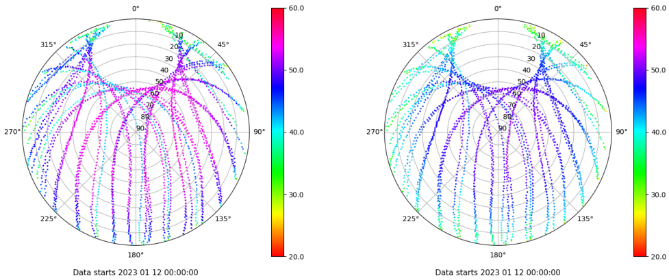
Skyplot for station SINE. Signal to Noise S1C Data file SINE00ESP_R_2023012.xtr Skyplot for station SINE. Signal to Noise S2P Data file SINE00ESP_R_2023012.xtr
