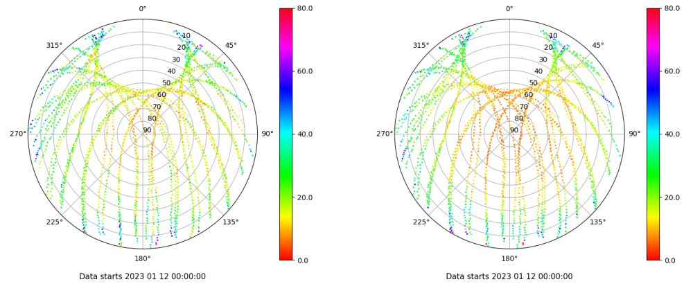
Skyplot for station SINE. Parameter M1C Data file SINE00ESP_R_2023012.xtr Skyplot for station SINE. Parameter M2P Data file SINE00ESP_R_2023012.xtr
