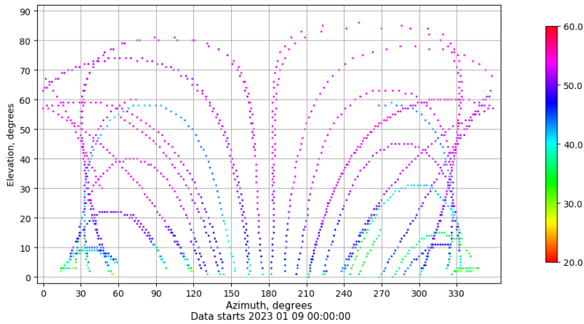
Azimuth-elevation plot for station SINE. Signal to Noise S1C Data file SINE00ESP_R_2023009.xtr
