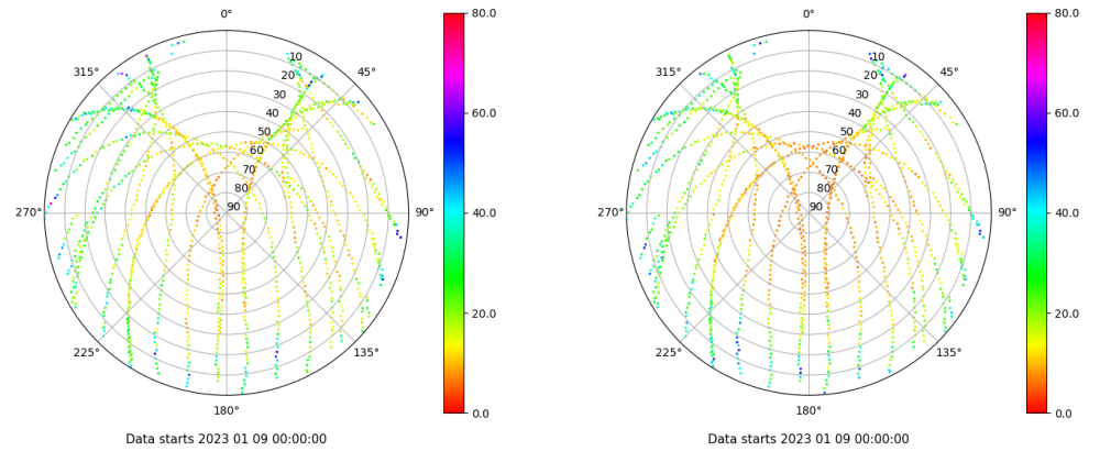
Skyplot for station SINE. Parameter M1C Data file SINE00ESP_R_2023009.xtr Skyplot for station SINE. Parameter M2P Data file SINE00ESP_R_2023009.xtr
