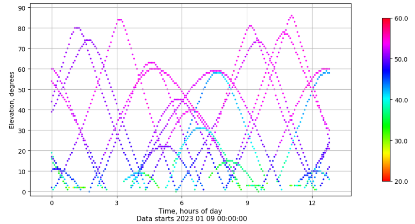
Time-elevation plot for station SINE. Signal to Noise S1C Data file SINE00ESP_R_2023009.xtr
