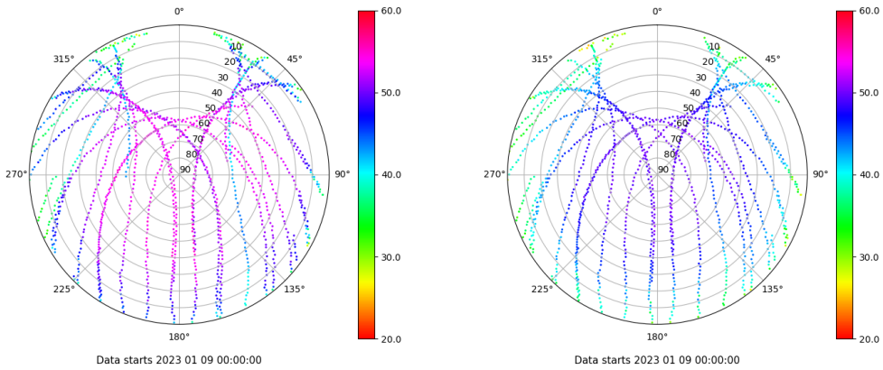
Skyplot for station SINE. Signal to Noise S1C Data file SINE00ESP_R_2023009.xtr Skyplot for station SINE. Signal to Noise S2P Data file SINE00ESP_R_2023009.xtr
