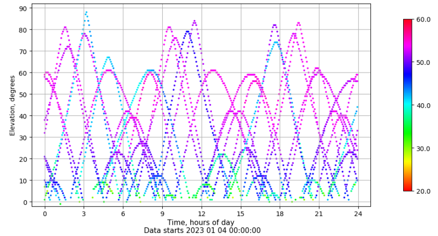
Time-elevation plot for station SINE. Signal to Noise S1C Data file SINE00ESP_R_2023004.xtr
