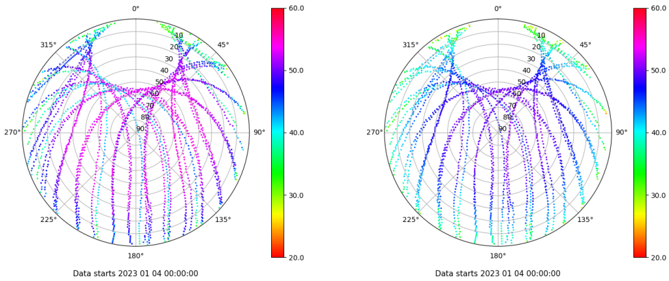
Skyplot for station SINE. Signal to Noise S1C Data file SINE00ESP_R_2023004.xtr Skyplot for station SINE. Signal to Noise S2P Data file SINE00ESP_R_2023004.xtr
