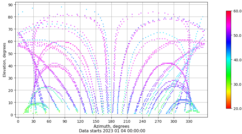
Azimuth-elevation plot for station SINE. Signal to Noise S1C Data file SINE00ESP_R_2023004.xtr
