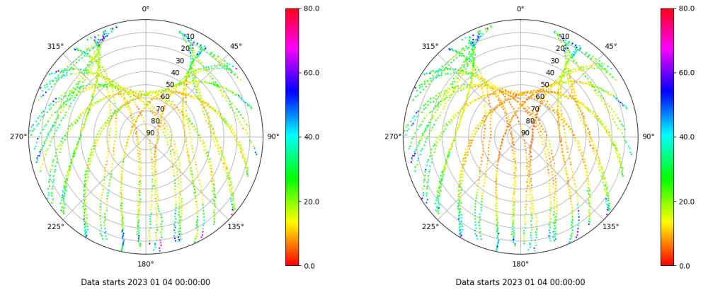
Skyplot for station SINE. Parameter M1C Data file SINE00ESP_R_2023004.xtr Skyplot for station SINE. Parameter M2P Data file SINE00ESP_R_2023004.xtr
