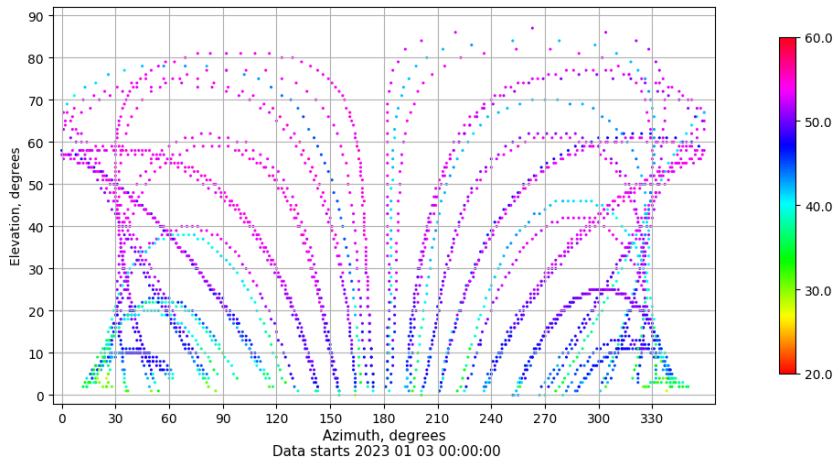
Azimuth-elevation plot for station SINE. Signal to Noise S1C Data file SINE00ESP_R_2023003.xtr
