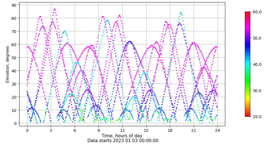
Time-elevation plot for station SINE. Signal to Noise S1C Data file SINE00ESP_R_2023003.xtr
