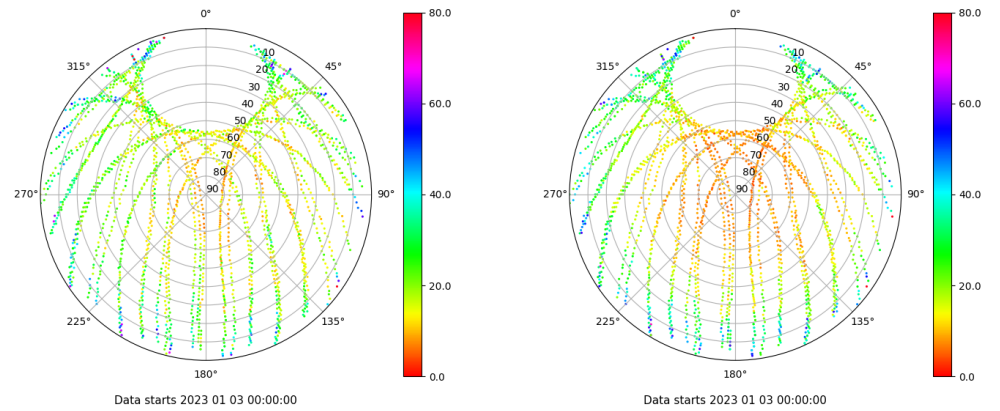
Skyplot for station SINE. Parameter M1C Data file SINE00ESP_R_2023003.xtr Skyplot for station SINE. Parameter M2P Data file SINE00ESP_R_2023003.xtr
