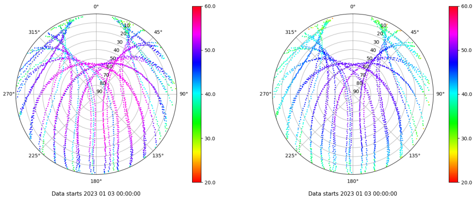
Skyplot for station SINE. Signal to Noise S1C Data file SINE00ESP_R_2023003.xtr Skyplot for station SINE. Signal to Noise S2P Data file SINE00ESP_R_2023003.xtr
