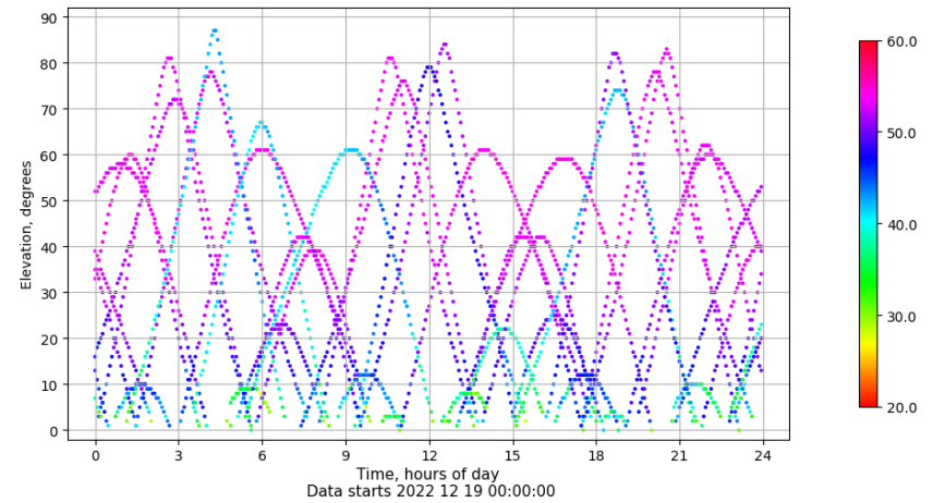
Time-elevation plot for station SINE. Signal to Noise S1C Data file SINE00ESP_R_2022353.xtr
