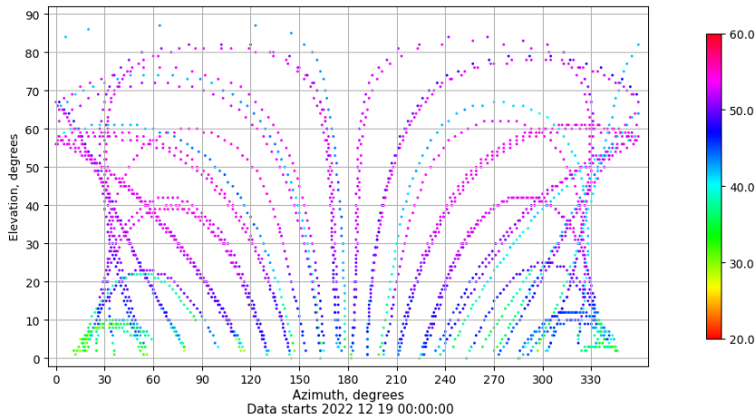
Azimuth-elevation plot for station SINE. Signal to Noise S1C Data file SINE00ESP_R_2022353.xtr
