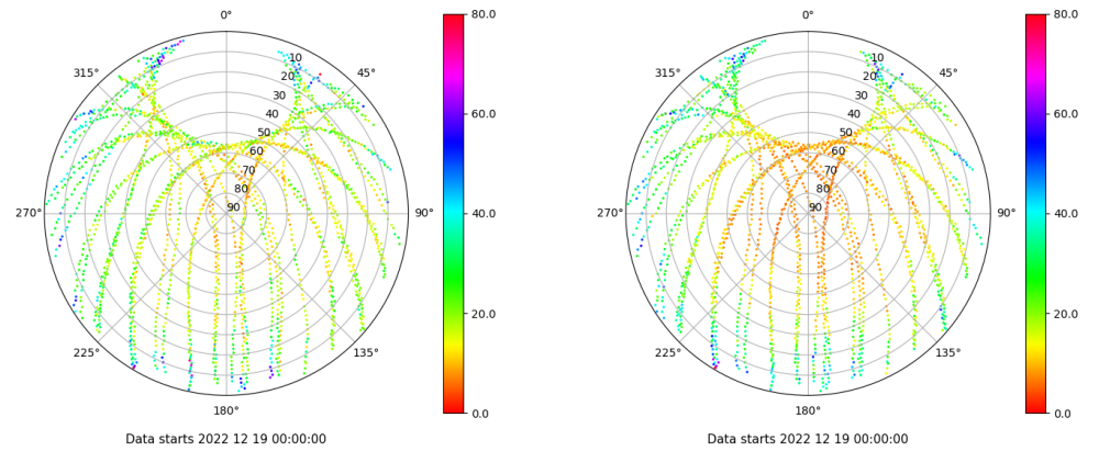
Skyplot for station SINE. Parameter M1C Data file SINE00ESP_R_2022353.xtr Skyplot for station SINE. Parameter M2P Data file SINE00ESP_R_2022353.xtr
