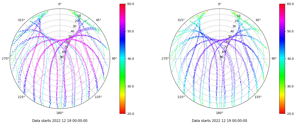
Skyplot for station SINE. Signal to Noise S1C Data file SINE00ESP_R_2022353.xtr Skyplot for station SINE. Signal to Noise S2P Data file SINE00ESP_R_2022353.xtr
