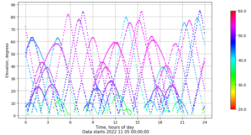
Time-elevation plot for station SINE. Signal to Noise S1C Data file SINE00ESP_R_2022309.xtr
