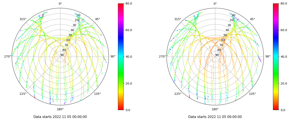
Skyplot for station SINE. Parameter M1C Data file SINE00ESP_R_2022309.xtr Skyplot for station SINE. Parameter M2P Data file SINE00ESP_R_2022309.xtr
