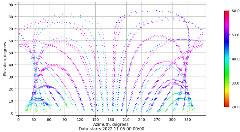
Azimuth-elevation plot for station SINE. Signal to Noise S1C Data file SINE00ESP_R_2022309.xtr
