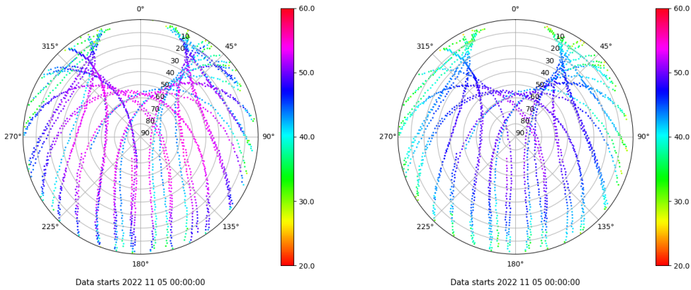
Skyplot for station SINE. Signal to Noise S1C Data file SINE00ESP_R_2022309.xtr Skyplot for station SINE. Signal to Noise S2P Data file SINE00ESP_R_2022309.xtr
