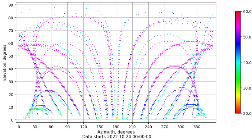
Azimuth-elevation plot for station SINE. Signal to Noise S1C Data file SINE00ESP_R_2022297.xtr
