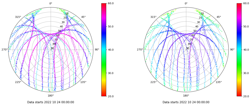
Skyplot for station SINE. Signal to Noise S1C Data file SINE00ESP_R_2022297.xtr Skyplot for station SINE. Signal to Noise S2P Data file SINE00ESP_R_2022297.xtr
