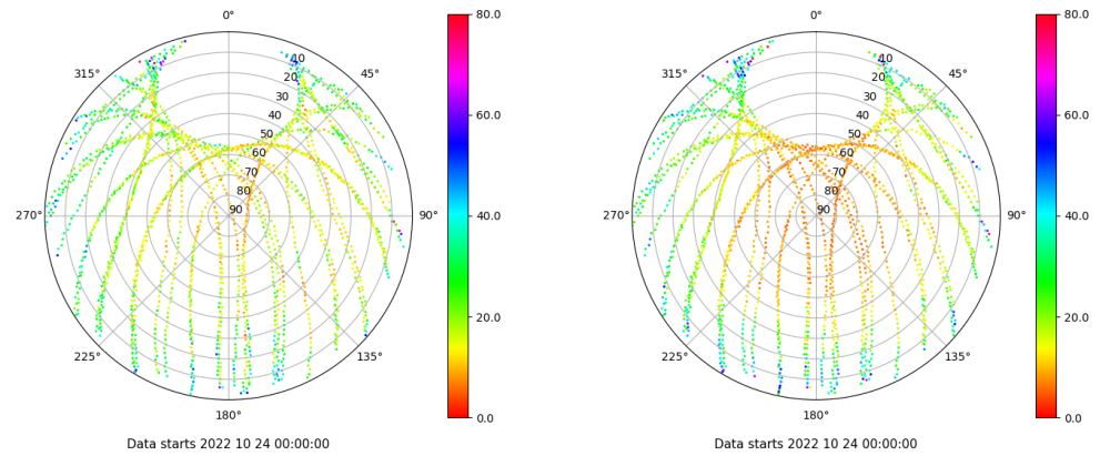
Skyplot for station SINE. Parameter M1C Data file SINE00ESP_R_2022297.xtr Skyplot for station SINE. Parameter M2P Data file SINE00ESP_R_2022297.xtr
