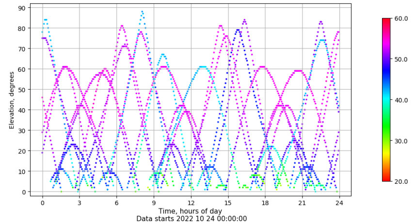
Time-elevation plot for station SINE. Signal to Noise S1C Data file SINE00ESP_R_2022297.xtr
