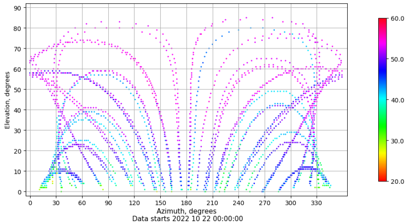
Azimuth-elevation plot for station SINE. Signal to Noise S1C Data file SINE00ESP_R_2022295.xtr
