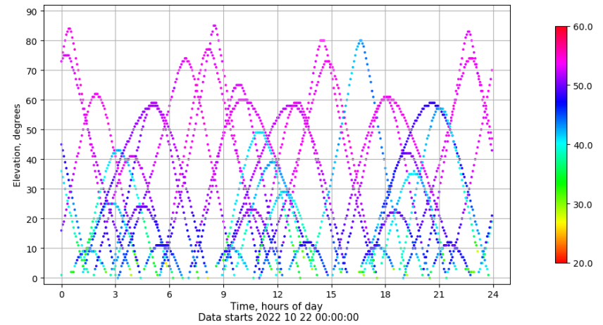
Time-elevation plot for station SINE. Signal to Noise S1C Data file SINE00ESP_R_2022295.xtr
