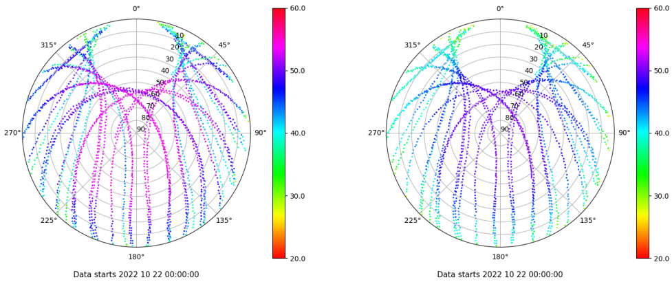
Skyplot for station SINE. Signal to Noise S1C Data file SINE00ESP_R_2022295.xtr Skyplot for station SINE. Signal to Noise S2P Data file SINE00ESP_R_2022295.xtr
