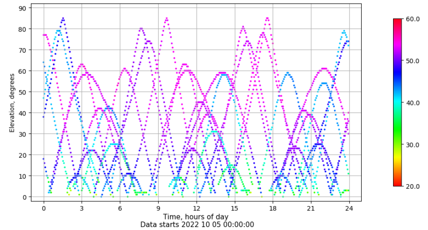
Time-elevation plot for station SINE. Signal to Noise S1C Data file SINE00ESP_R_2022278.xtr
