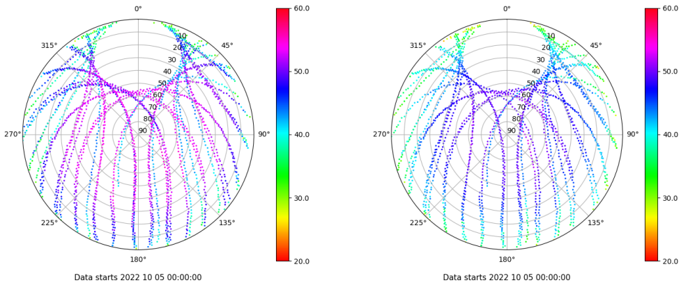
Skyplot for station SINE. Signal to Noise S1C Data file SINE00ESP_R_2022278.xtr Skyplot for station SINE. Signal to Noise S2P Data file SINE00ESP_R_2022278.xtr
