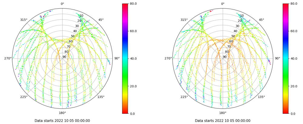
Skyplot for station SINE. Parameter M1C Data file SINE00ESP_R_2022278.xtr Skyplot for station SINE. Parameter M2P Data file SINE00ESP_R_2022278.xtr
