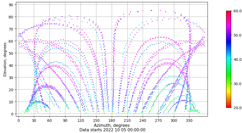
Azimuth-elevation plot for station SINE. Signal to Noise S1C Data file SINE00ESP_R_2022278.xtr
