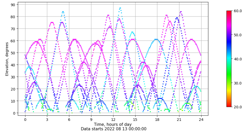
Time-elevation plot for station SINE. Signal to Noise S1C Data file SINE00ESP_R_2022225.xtr
