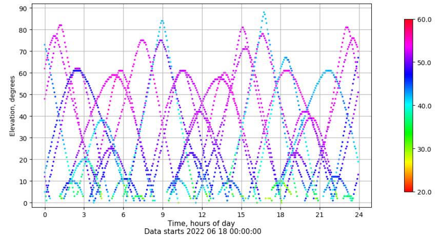
Time-elevation plot for station SINE. Signal to Noise S1C Data file SINE00ESP_R_2022169.xtr
