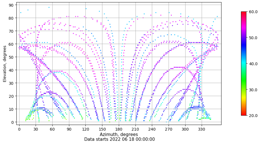
Azimuth-elevation plot for station SINE. Signal to Noise S1C Data file SINE00ESP_R_2022169.xtr
