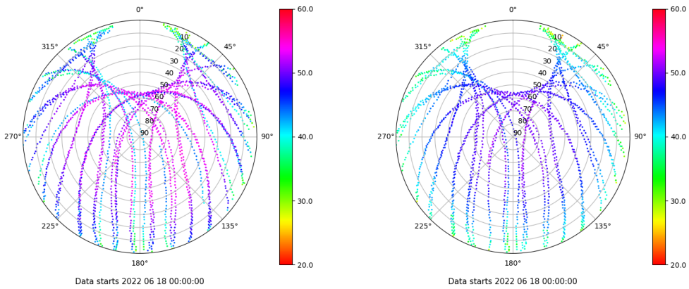
Skyplot for station SINE. Signal to Noise S1C Data file SINE00ESP_R_2022169.xtr Skyplot for station SINE. Signal to Noise S2P Data file SINE00ESP_R_2022169.xtr
