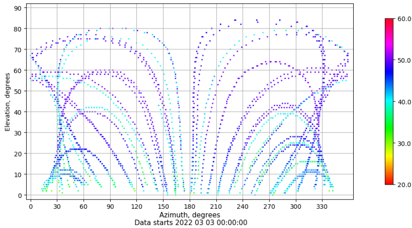
Azimuth-elevation plot for station SINE. Signal to Noise S1C Data file SINE00ESP_R_2022062.xtr
