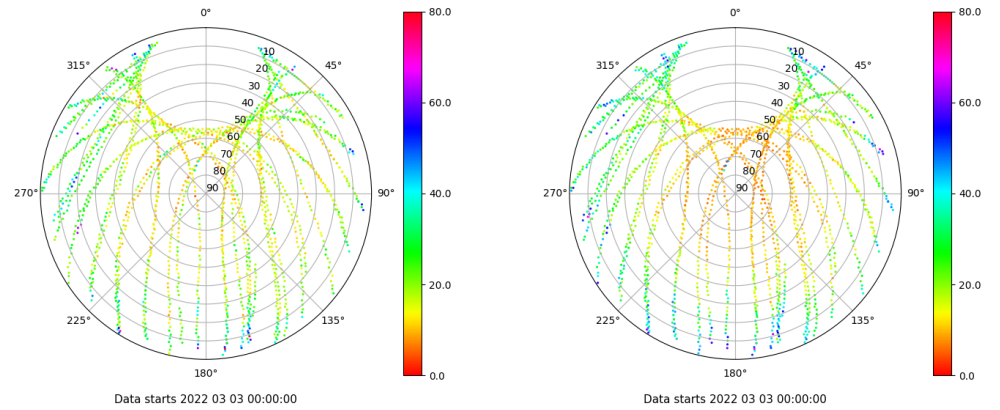
Skyplot for station SINE. Parameter M1C Data file SINE00ESP_R_2022062.xtr Skyplot for station SINE. Parameter M2P Data file SINE00ESP_R_2022062.xtr
