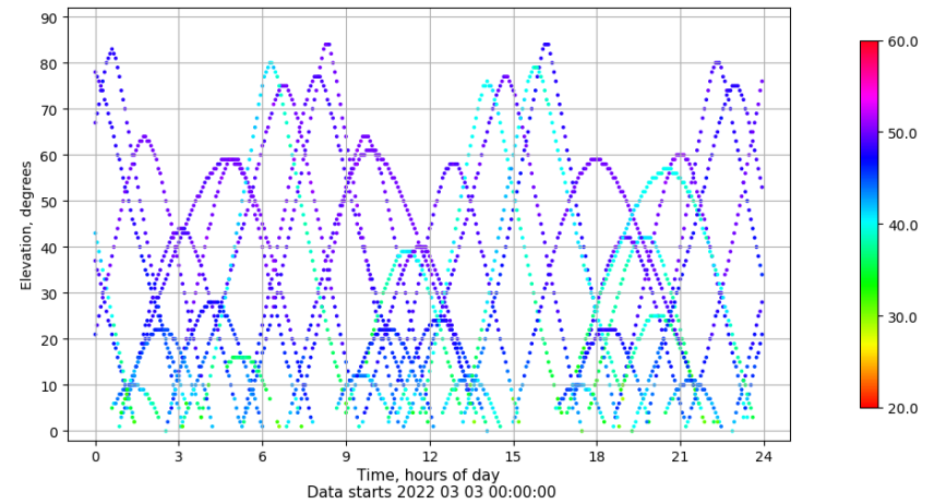
Time-elevation plot for station SINE. Signal to Noise S1C Data file SINE00ESP_R_2022062.xtr
