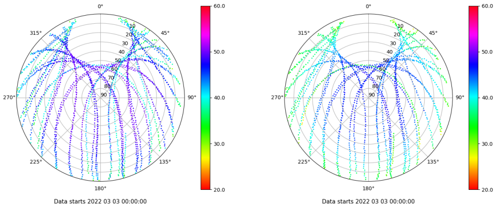
Skyplot for station SINE. Signal to Noise S1C Data file SINE00ESP_R_2022062.xtr Skyplot for station SINE. Signal to Noise S2P Data file SINE00ESP_R_2022062.xtr
