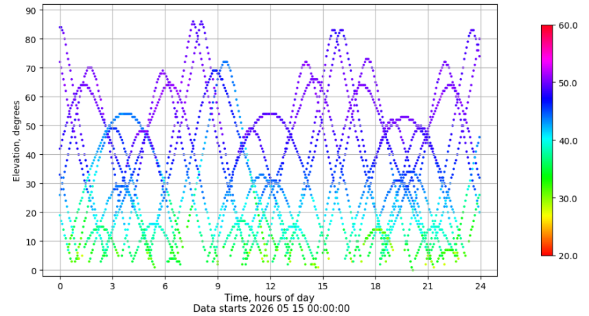
Time-elevation plot for station SEV1. Signal to Noise S1C Data file SEV100ESP_R_2026135.xtr
