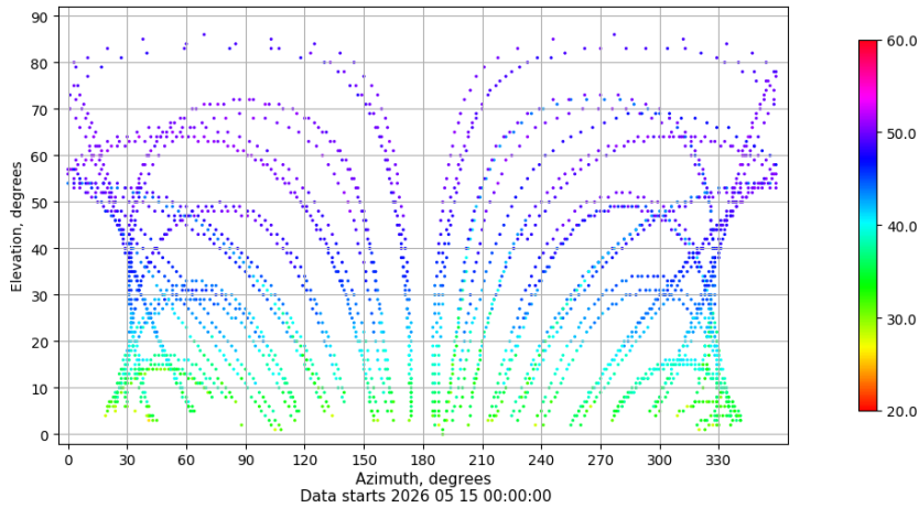
Azimuth-elevation plot for station SEV1. Signal to Noise S1C Data file SEV100ESP_R_2026135.xtr
