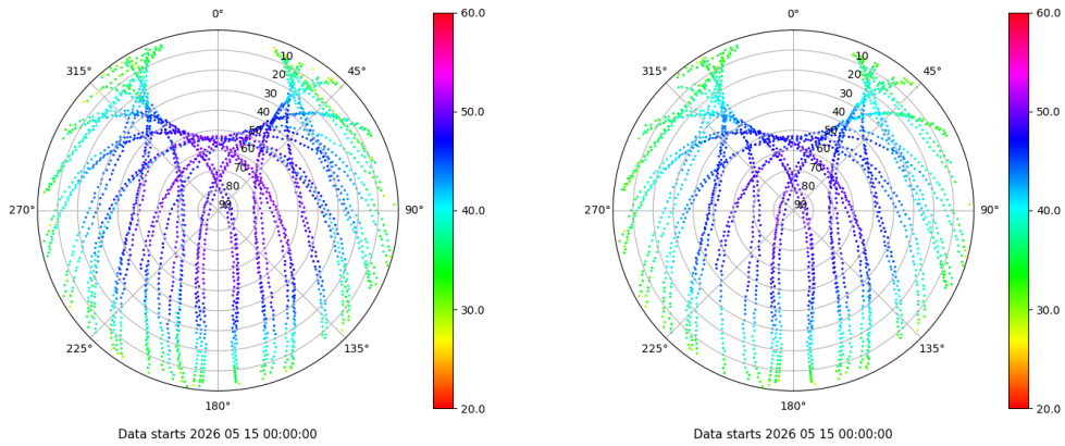
Skyplot for station SEV1. Signal to Noise S1C Data file SEV100ESP_R_2026135.xtr Skyplot for station SEV1. Signal to Noise S2C Data file SEV100ESP_R_2026135.xtr
