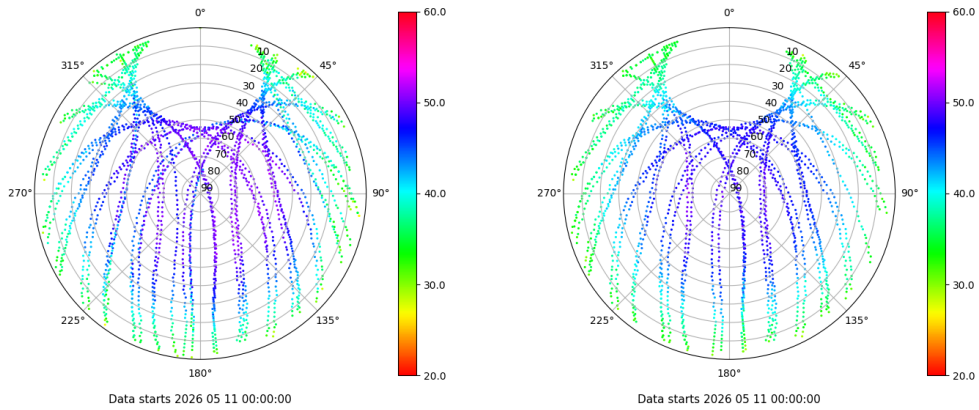
Skyplot for station SEV1. Signal to Noise S1C Data file SEV100ESP_R_2026131.xtr Skyplot for station SEV1. Signal to Noise S2C Data file SEV100ESP_R_2026131.xtr
