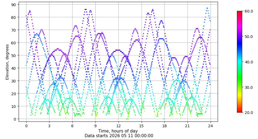
Time-elevation plot for station SEV1. Signal to Noise S1C Data file SEV100ESP_R_2026131.xtr
