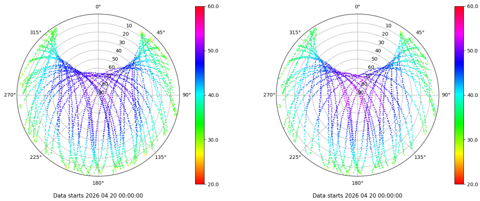
Skyplot for station SEV1. Signal to Noise S1C Data file SEV100ESP_R_2026110.xtr Skyplot for station SEV1. Signal to Noise S2X Data file SEV100ESP_R_2026110.xtr
