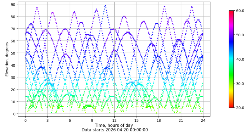
Time-elevation plot for station SEV1. Signal to Noise S1C Data file SEV100ESP_R_2026110.xtr
