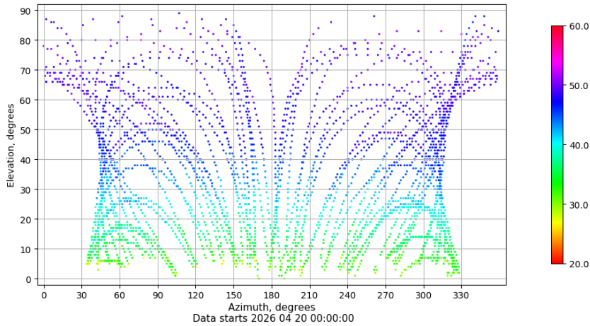
Azimuth-elevation plot for station SEV1. Signal to Noise S1C Data file SEV100ESP_R_2026110.xtr
