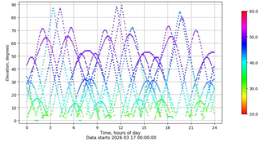
Time-elevation plot for station SEV1. Signal to Noise S1C Data file SEV100ESP_R_2026076.xtr
