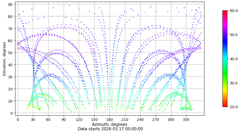
Azimuth-elevation plot for station SEV1. Signal to Noise S1C Data file SEV100ESP_R_2026076.xtr
