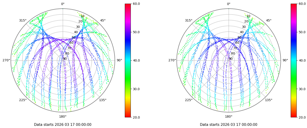
Skyplot for station SEV1. Signal to Noise S1C Data file SEV100ESP_R_2026076.xtr Skyplot for station SEV1. Signal to Noise S2C Data file SEV100ESP_R_2026076.xtr
