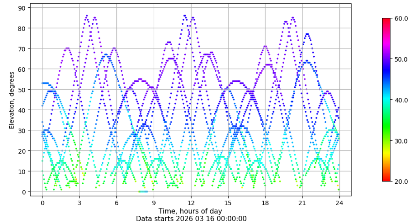
Time-elevation plot for station SEV1. Signal to Noise S1C Data file SEV100ESP_R_2026075.xtr
