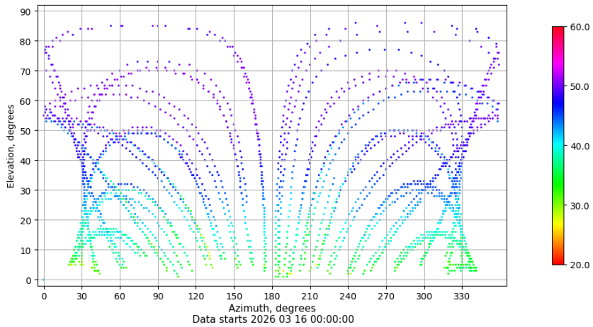
Azimuth-elevation plot for station SEV1. Signal to Noise S1C Data file SEV100ESP_R_2026075.xtr
