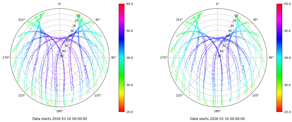
Skyplot for station SEV1. Signal to Noise S1C Data file SEV100ESP_R_2026075.xtr Skyplot for station SEV1. Signal to Noise S2C Data file SEV100ESP_R_2026075.xtr
