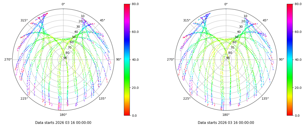
Skyplot for station SEV1. Parameter M1C Data file SEV100ESP_R_2026075.xtr Skyplot for station SEV1. Parameter M2C Data file SEV100ESP_R_2026075.xtr
