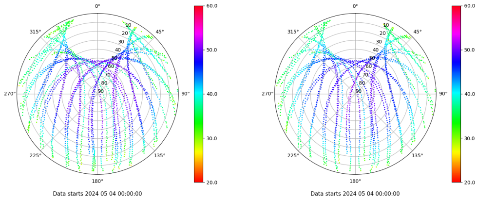
Skyplot for station SEV1. Signal to Noise S1C Data file SEV100ESP_R_2024125.xtr Skyplot for station SEV1. Signal to Noise S2C Data file SEV100ESP_R_2024125.xtr
