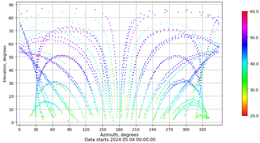
Azimuth-elevation plot for station SEV1. Signal to Noise S1C Data file SEV100ESP_R_2024125.xtr
