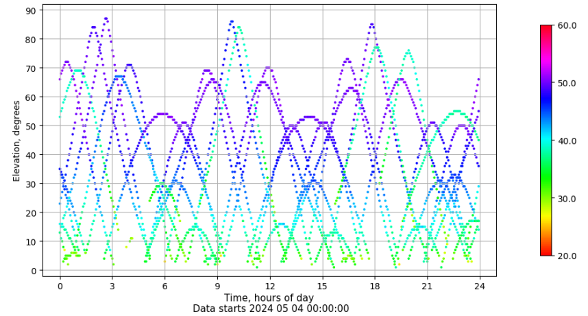
Time-elevation plot for station SEV1. Signal to Noise S1C Data file SEV100ESP_R_2024125.xtr
