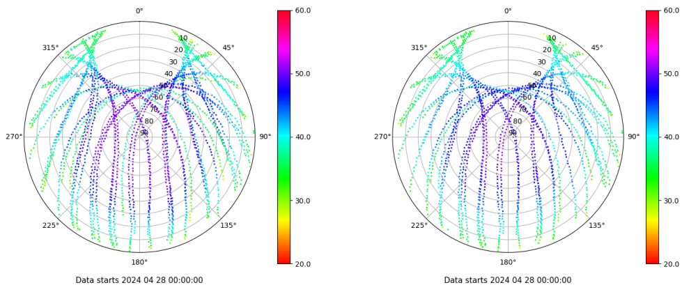
Skyplot for station SEV1. Signal to Noise S1C Data file SEV100ESP_R_2024119.xtr Skyplot for station SEV1. Signal to Noise S2C Data file SEV100ESP_R_2024119.xtr
