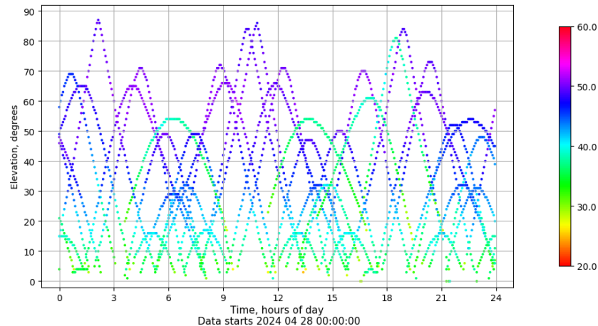
Time-elevation plot for station SEV1. Signal to Noise S1C Data file SEV100ESP_R_2024119.xtr
