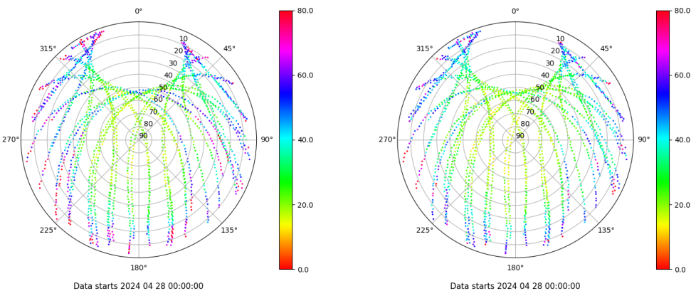
Skyplot for station SEV1. Parameter M1C Data file SEV100ESP_R_2024119.xtr Skyplot for station SEV1. Parameter M2C Data file SEV100ESP_R_2024119.xtr
