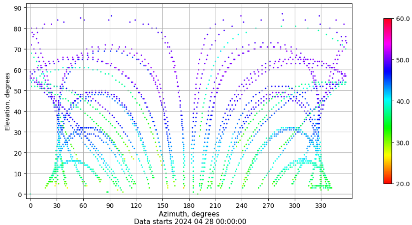
Azimuth-elevation plot for station SEV1. Signal to Noise S1C Data file SEV100ESP_R_2024119.xtr
