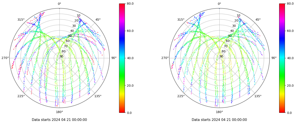
Skyplot for station SEV1. Parameter M1C Data file SEV100ESP_R_2024112.xtr Skyplot for station SEV1. Parameter M2C Data file SEV100ESP_R_2024112.xtr
