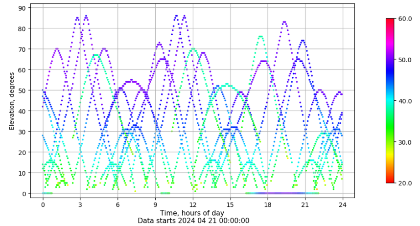
Time-elevation plot for station SEV1. Signal to Noise S1C Data file SEV100ESP_R_2024112.xtr
