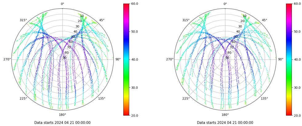
Skyplot for station SEV1. Signal to Noise S1C Data file SEV100ESP_R_2024112.xtr Skyplot for station SEV1. Signal to Noise S2C Data file SEV100ESP_R_2024112.xtr
