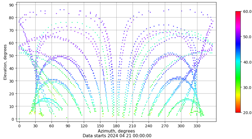
Azimuth-elevation plot for station SEV1. Signal to Noise S1C Data file SEV100ESP_R_2024112.xtr
