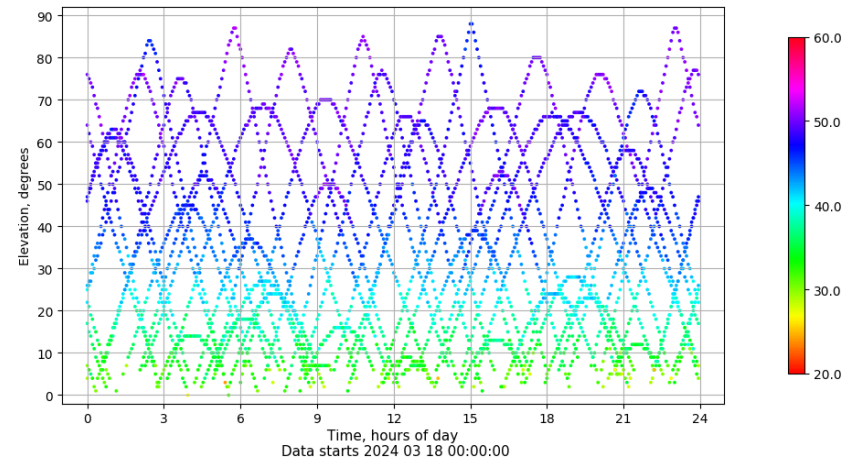
Time-elevation plot for station SEV1. Signal to Noise S1C Data file SEV100ESP_R_2024078.xtr
