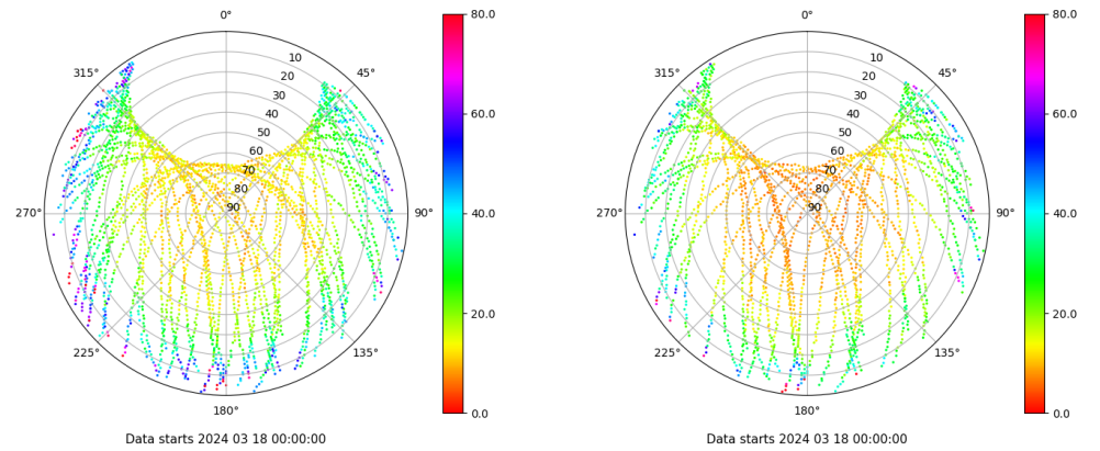
Skyplot for station SEV1. Parameter M1C Data file SEV100ESP_R_2024078.xtr Skyplot for station SEV1. Parameter M2X Data file SEV100ESP_R_2024078.xtr
