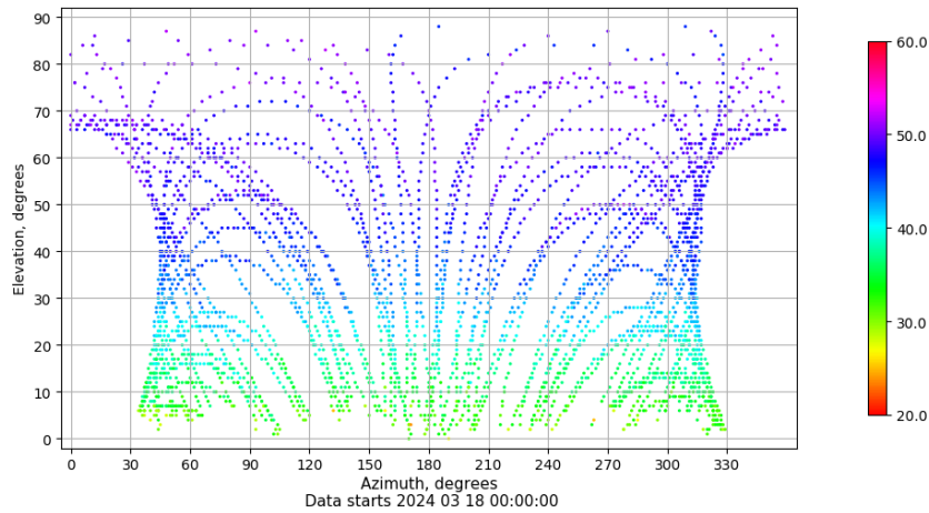
Azimuth-elevation plot for station SEV1. Signal to Noise S1C Data file SEV100ESP_R_2024078.xtr
