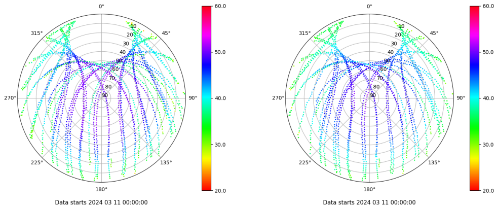
Skyplot for station SEV1. Signal to Noise S1C Data file SEV100ESP_R_2024071.xtr Skyplot for station SEV1. Signal to Noise S2C Data file SEV100ESP_R_2024071.xtr
