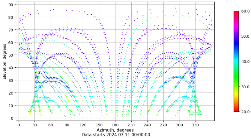
Azimuth-elevation plot for station SEV1. Signal to Noise S1C Data file SEV100ESP_R_2024071.xtr
