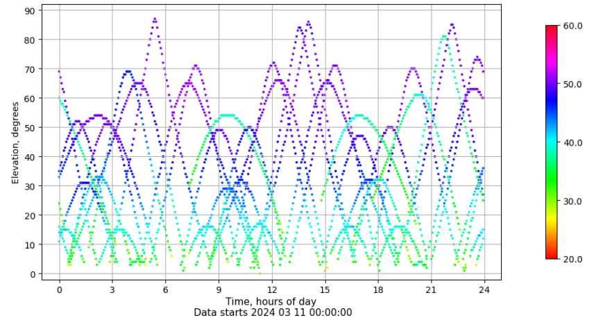
Time-elevation plot for station SEV1. Signal to Noise S1C Data file SEV100ESP_R_2024071.xtr
