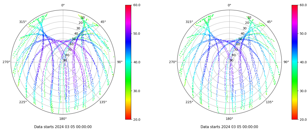
Skyplot for station SEV1. Signal to Noise S1C Data file SEV100ESP_R_2024065.xtr Skyplot for station SEV1. Signal to Noise S2C Data file SEV100ESP_R_2024065.xtr
