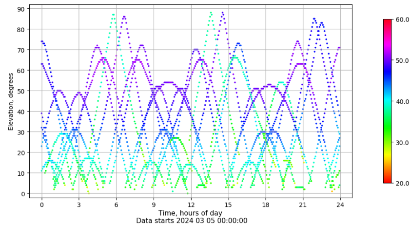
Time-elevation plot for station SEV1. Signal to Noise S1C Data file SEV100ESP_R_2024065.xtr
