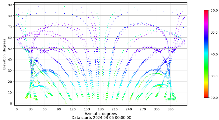
Azimuth-elevation plot for station SEV1. Signal to Noise S1C Data file SEV100ESP_R_2024065.xtr
