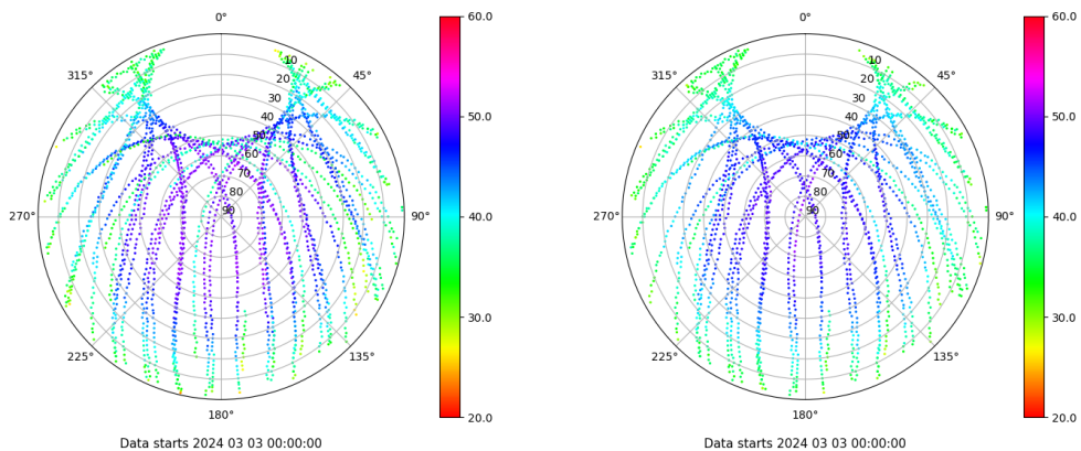
Skyplot for station SEV1. Signal to Noise S1C Data file SEV100ESP_R_2024063.xtr Skyplot for station SEV1. Signal to Noise S2C Data file SEV100ESP_R_2024063.xtr
