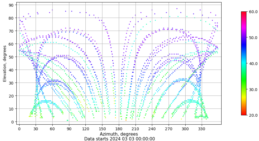
Azimuth-elevation plot for station SEV1. Signal to Noise S1C Data file SEV100ESP_R_2024063.xtr
