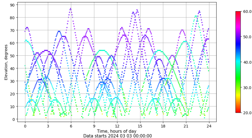
Time-elevation plot for station SEV1. Signal to Noise S1C Data file SEV100ESP_R_2024063.xtr
