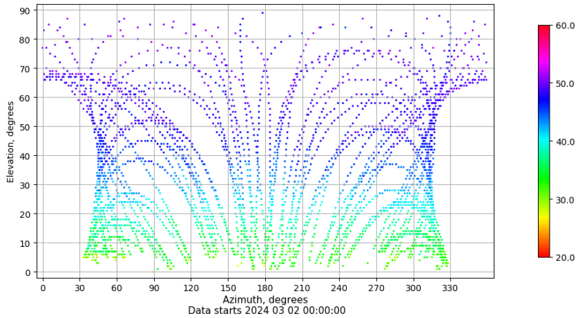
Azimuth-elevation plot for station SEV1. Signal to Noise S1C Data file SEV100ESP_R_2024062.xtr
