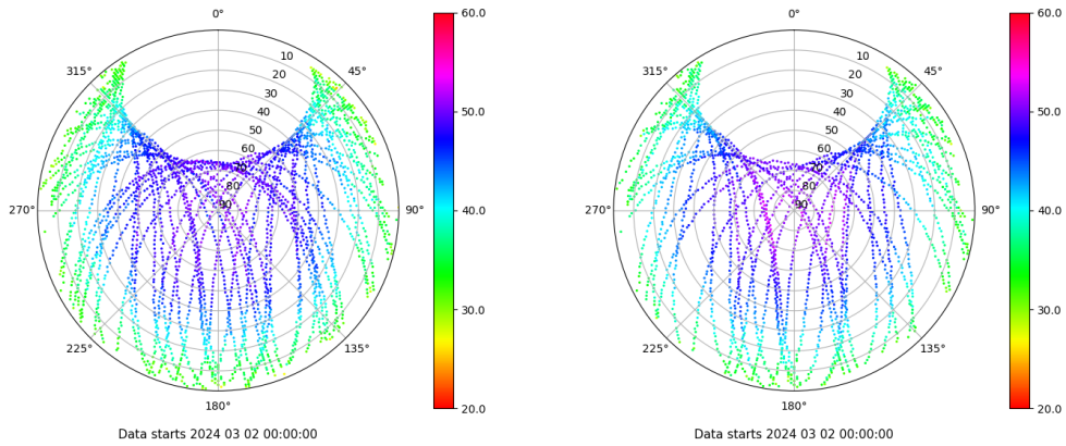
Skyplot for station SEV1. Signal to Noise S1C Data file SEV100ESP_R_2024062.xtr Skyplot for station SEV1. Signal to Noise S2X Data file SEV100ESP_R_2024062.xtr
