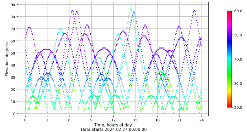
Time-elevation plot for station SEV1. Signal to Noise S1C Data file SEV100ESP_R_2024058.xtr
