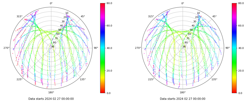
Skyplot for station SEV1. Parameter M1C Data file SEV100ESP_R_2024058.xtr Skyplot for station SEV1. Parameter M2C Data file SEV100ESP_R_2024058.xtr
