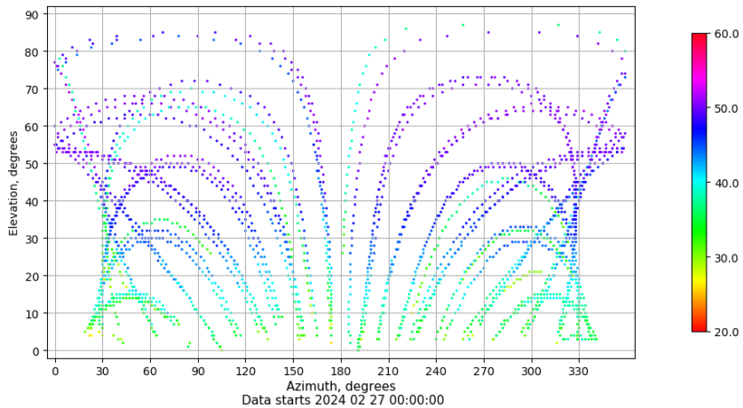
Azimuth-elevation plot for station SEV1. Signal to Noise S1C Data file SEV100ESP_R_2024058.xtr
