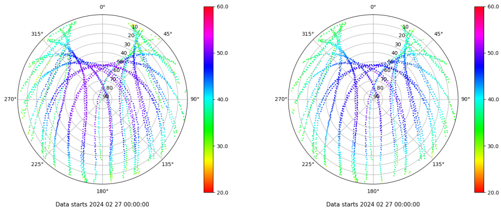
Skyplot for station SEV1. Signal to Noise S1C Data file SEV100ESP_R_2024058.xtr Skyplot for station SEV1. Signal to Noise S2C Data file SEV100ESP_R_2024058.xtr
