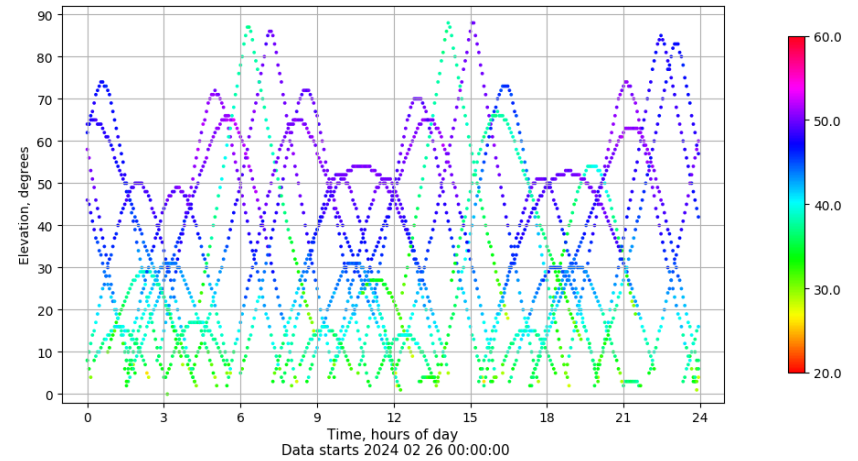
Time-elevation plot for station SEV1. Signal to Noise S1C Data file SEV100ESP_R_2024057.xtr
