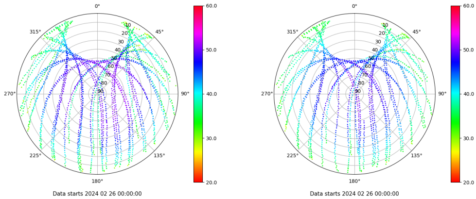
Skyplot for station SEV1. Signal to Noise S1C Data file SEV100ESP_R_2024057.xtr Skyplot for station SEV1. Signal to Noise S2C Data file SEV100ESP_R_2024057.xtr
