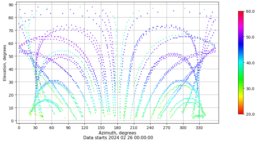
Azimuth-elevation plot for station SEV1. Signal to Noise S1C Data file SEV100ESP_R_2024057.xtr
