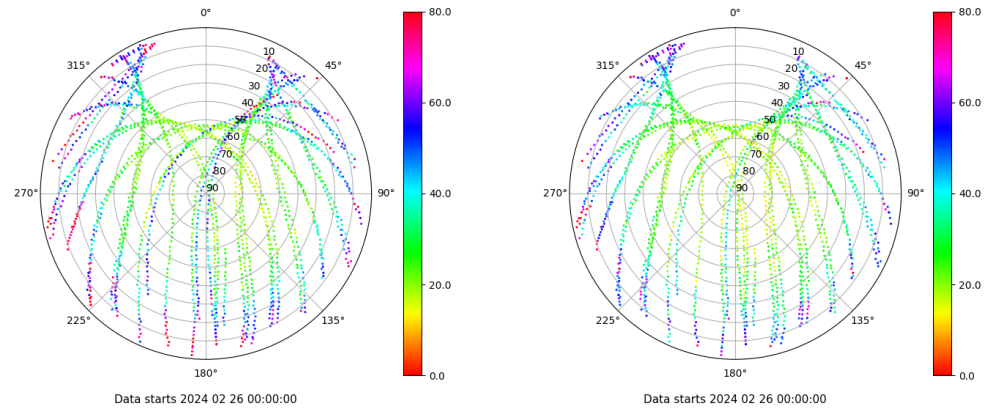
Skyplot for station SEV1. Parameter M1C Data file SEV100ESP_R_2024057.xtr Skyplot for station SEV1. Parameter M2C Data file SEV100ESP_R_2024057.xtr
