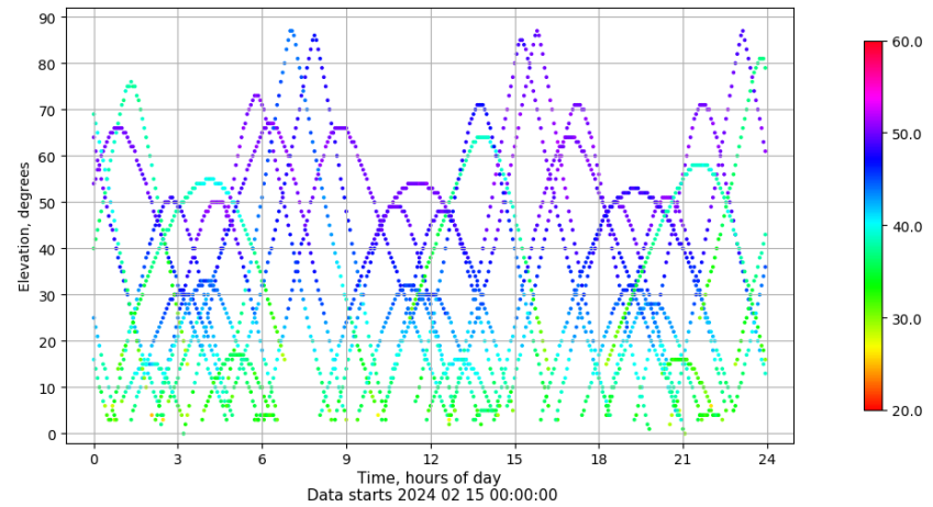
Time-elevation plot for station SEV1. Signal to Noise S1C Data file SEV100ESP_R_2024046.xtr
