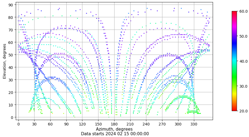
Azimuth-elevation plot for station SEV1. Signal to Noise S1C Data file SEV100ESP_R_2024046.xtr
