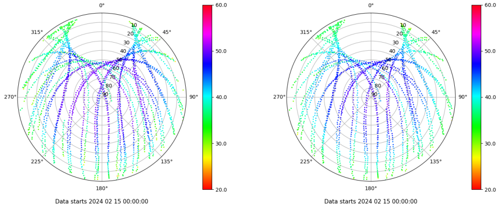
Skyplot for station SEV1. Signal to Noise S1C Data file SEV100ESP_R_2024046.xtr Skyplot for station SEV1. Signal to Noise S2C Data file SEV100ESP_R_2024046.xtr
