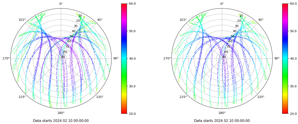
Skyplot for station SEV1. Signal to Noise S1C Data file SEV100ESP_R_2024041.xtr Skyplot for station SEV1. Signal to Noise S2C Data file SEV100ESP_R_2024041.xtr
