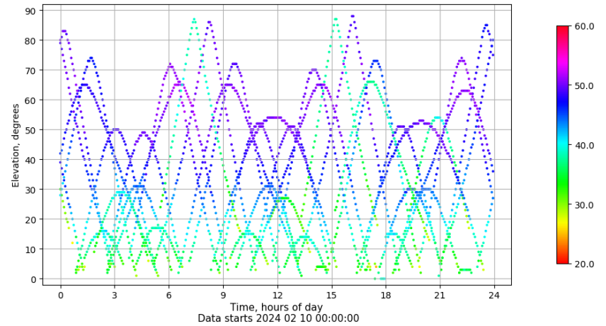
Time-elevation plot for station SEV1. Signal to Noise S1C Data file SEV100ESP_R_2024041.xtr
