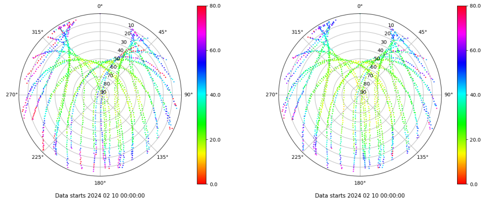
Skyplot for station SEV1. Parameter M1C Data file SEV100ESP_R_2024041.xtr Skyplot for station SEV1. Parameter M2C Data file SEV100ESP_R_2024041.xtr
