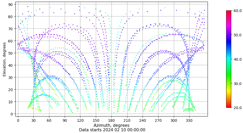
Azimuth-elevation plot for station SEV1. Signal to Noise S1C Data file SEV100ESP_R_2024041.xtr
