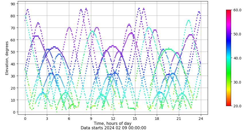
Time-elevation plot for station SEV1. Signal to Noise S1C Data file SEV100ESP_R_2024040.xtr
