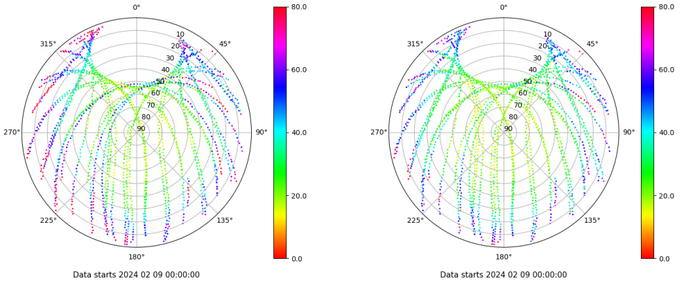
Skyplot for station SEV1. Parameter M1C Data file SEV100ESP_R_2024040.xtr Skyplot for station SEV1. Parameter M2C Data file SEV100ESP_R_2024040.xtr
