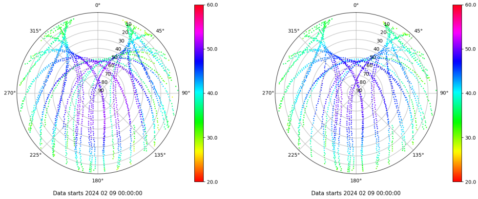
Skyplot for station SEV1. Signal to Noise S1C Data file SEV100ESP_R_2024040.xtr Skyplot for station SEV1. Signal to Noise S2C Data file SEV100ESP_R_2024040.xtr
