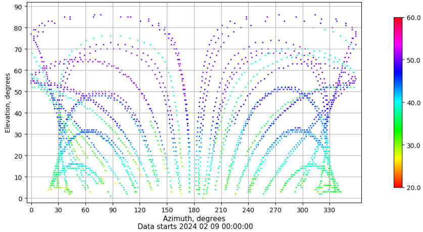
Azimuth-elevation plot for station SEV1. Signal to Noise S1C Data file SEV100ESP_R_2024040.xtr
