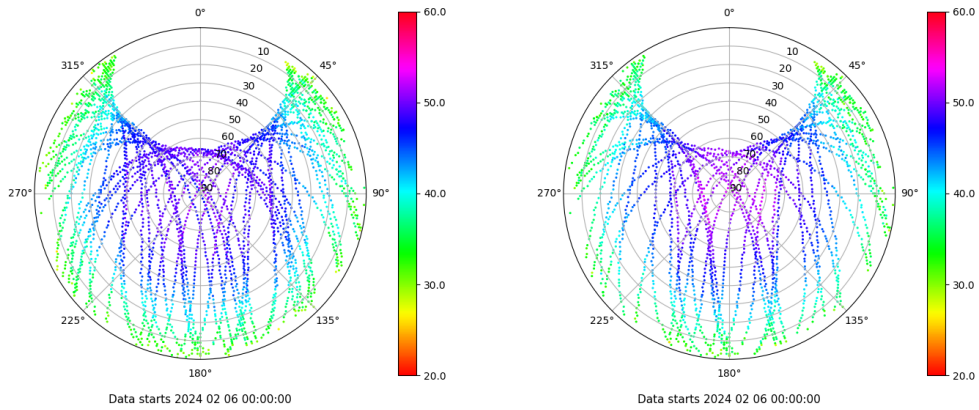
Skyplot for station SEV1. Signal to Noise S1C Data file SEV100ESP_R_2024037.xtr Skyplot for station SEV1. Signal to Noise S2X Data file SEV100ESP_R_2024037.xtr
