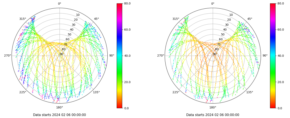
Skyplot for station SEV1. Parameter M1C Data file SEV100ESP_R_2024037.xtr Skyplot for station SEV1. Parameter M2X Data file SEV100ESP_R_2024037.xtr
