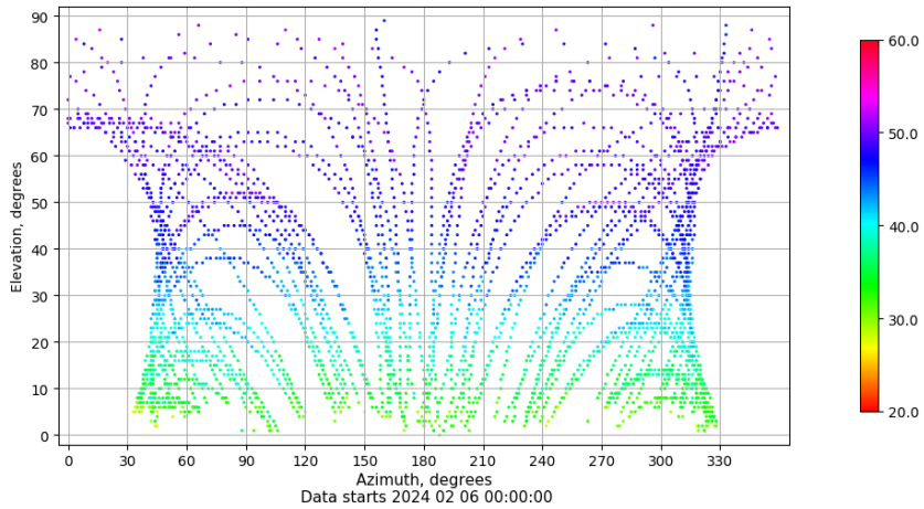
Azimuth-elevation plot for station SEV1. Signal to Noise S1C Data file SEV100ESP_R_2024037.xtr
