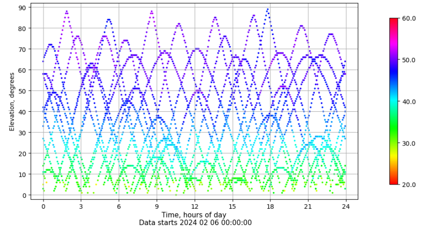
Time-elevation plot for station SEV1. Signal to Noise S1C Data file SEV100ESP_R_2024037.xtr
