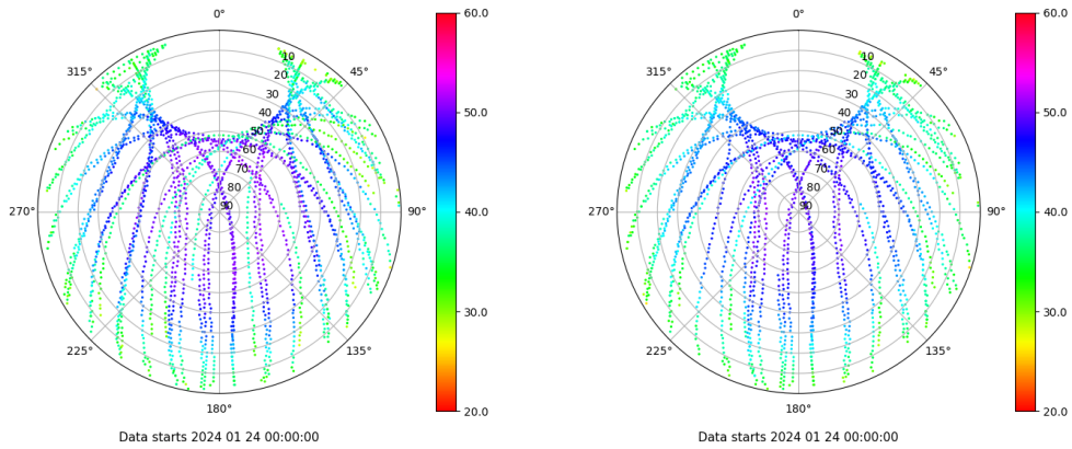
Skyplot for station SEV1. Signal to Noise S1C Data file SEV100ESP_R_2024024.xtr Skyplot for station SEV1. Signal to Noise S2C Data file SEV100ESP_R_2024024.xtr
