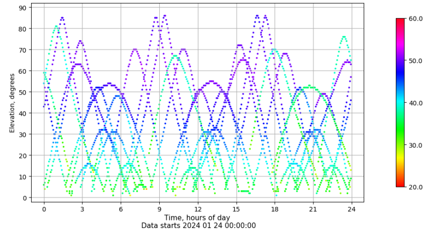
Time-elevation plot for station SEV1. Signal to Noise S1C Data file SEV100ESP_R_2024024.xtr
