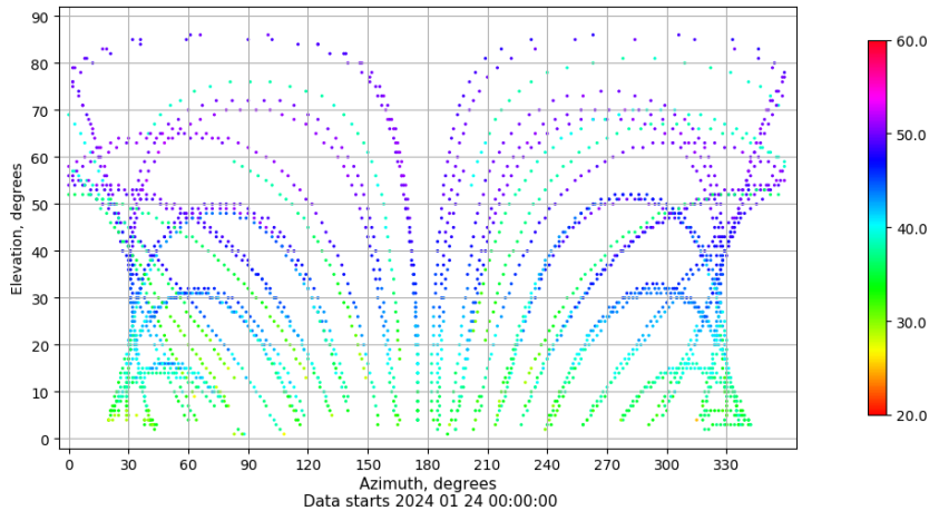
Azimuth-elevation plot for station SEV1. Signal to Noise S1C Data file SEV100ESP_R_2024024.xtr
