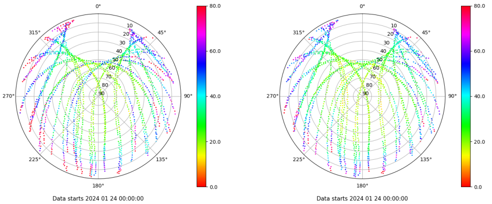
Skyplot for station SEV1. Parameter M1C Data file SEV100ESP_R_2024024.xtr Skyplot for station SEV1. Parameter M2C Data file SEV100ESP_R_2024024.xtr
