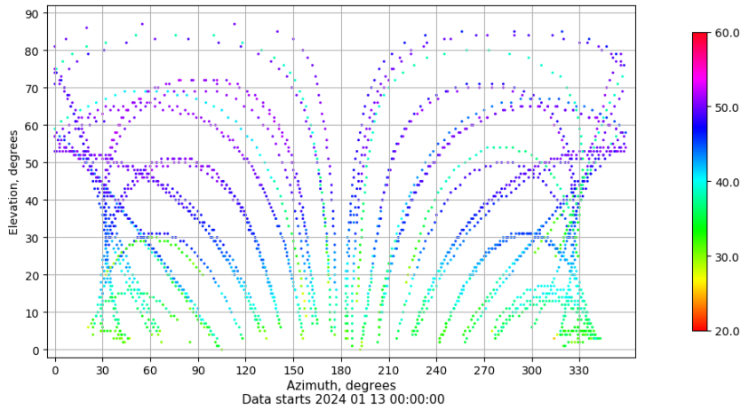
Azimuth-elevation plot for station SEV1. Signal to Noise S1C Data file SEV100ESP_R_2024013.xtr
