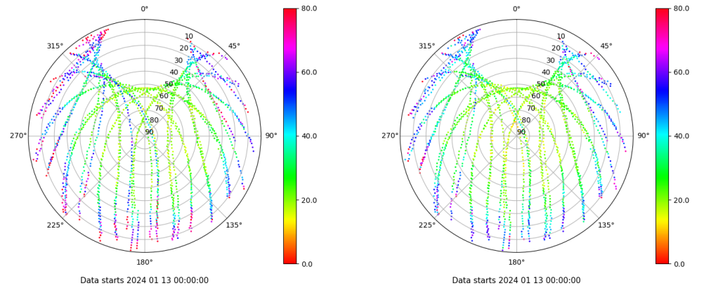
Skyplot for station SEV1. Parameter M1C Data file SEV100ESP_R_2024013.xtr Skyplot for station SEV1. Parameter M2C Data file SEV100ESP_R_2024013.xtr
