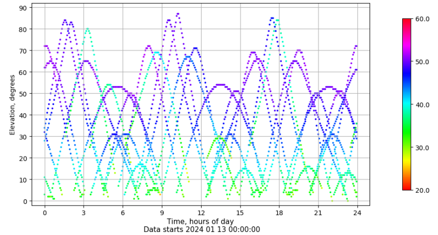
Time-elevation plot for station SEV1. Signal to Noise S1C Data file SEV100ESP_R_2024013.xtr
