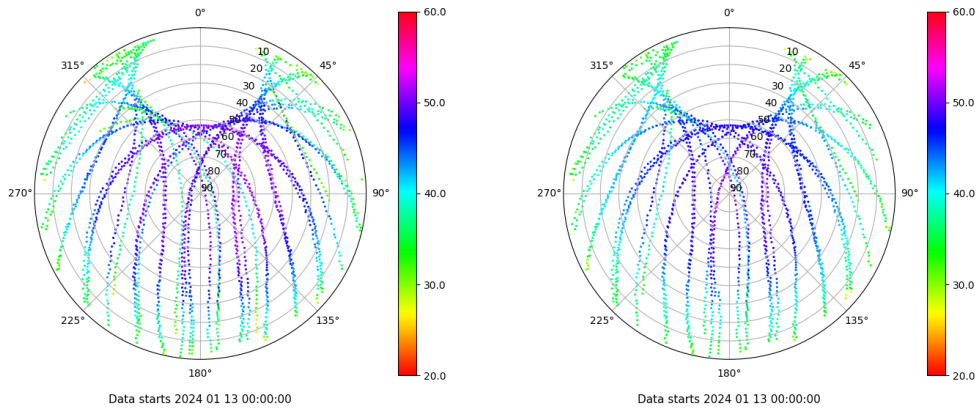
Skyplot for station SEV1. Signal to Noise S1C Data file SEV100ESP_R_2024013.xtr Skyplot for station SEV1. Signal to Noise S2C Data file SEV100ESP_R_2024013.xtr
