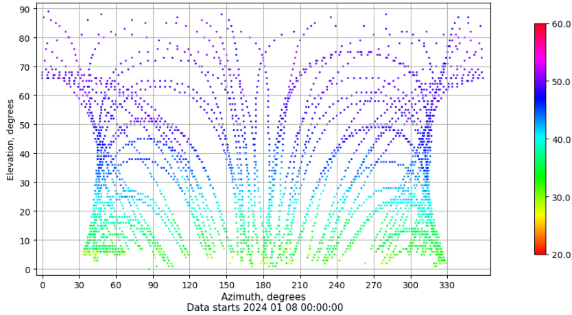
Azimuth-elevation plot for station SEV1. Signal to Noise S1C Data file SEV100ESP_R_2024008.xtr
