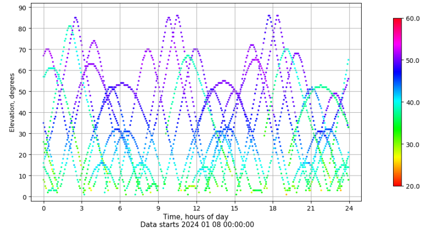
Time-elevation plot for station SEV1. Signal to Noise S1C Data file SEV100ESP_R_2024008.xtr
