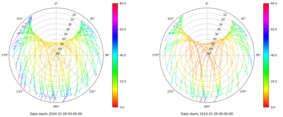
Skyplot for station SEV1. Parameter M1C Data file SEV100ESP_R_2024008.xtr Skyplot for station SEV1. Parameter M2X Data file SEV100ESP_R_2024008.xtr
