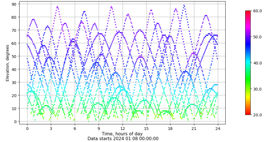
Time-elevation plot for station SEV1. Signal to Noise S1C Data file SEV100ESP_R_2024008.xtr
