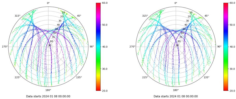
Skyplot for station SEV1. Signal to Noise S1C Data file SEV100ESP_R_2024008.xtr Skyplot for station SEV1. Signal to Noise S2C Data file SEV100ESP_R_2024008.xtr
