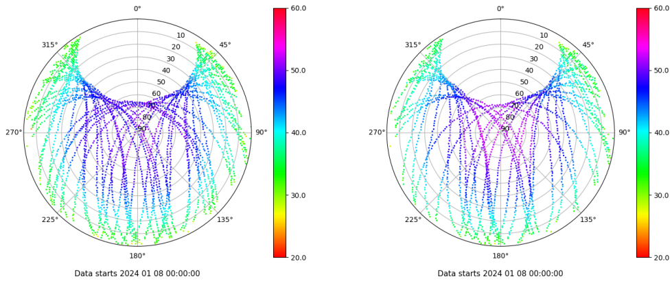
Skyplot for station SEV1. Signal to Noise S1C Data file SEV100ESP_R_2024008.xtr Skyplot for station SEV1. Signal to Noise S2X Data file SEV100ESP_R_2024008.xtr
