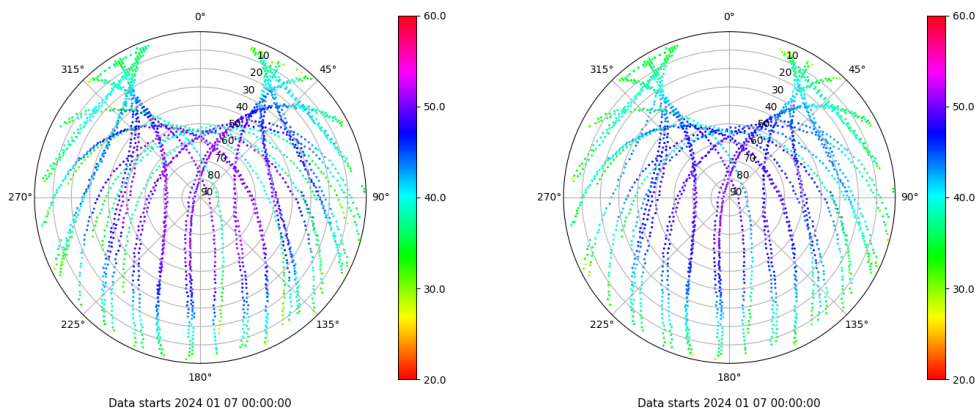
Skyplot for station SEV1. Signal to Noise S1C Data file SEV100ESP_R_2024007.xtr Skyplot for station SEV1. Signal to Noise S2C Data file SEV100ESP_R_2024007.xtr
