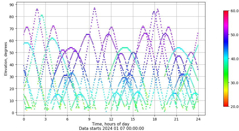
Time-elevation plot for station SEV1. Signal to Noise S1C Data file SEV100ESP_R_2024007.xtr
