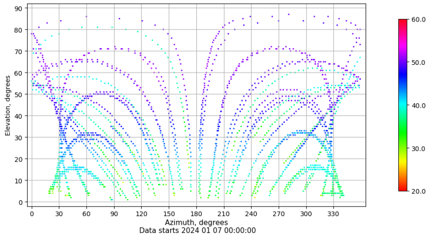
Azimuth-elevation plot for station SEV1. Signal to Noise S1C Data file SEV100ESP_R_2024007.xtr
