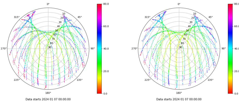
Skyplot for station SEV1. Parameter M1C Data file SEV100ESP_R_2024007.xtr Skyplot for station SEV1. Parameter M2C Data file SEV100ESP_R_2024007.xtr
