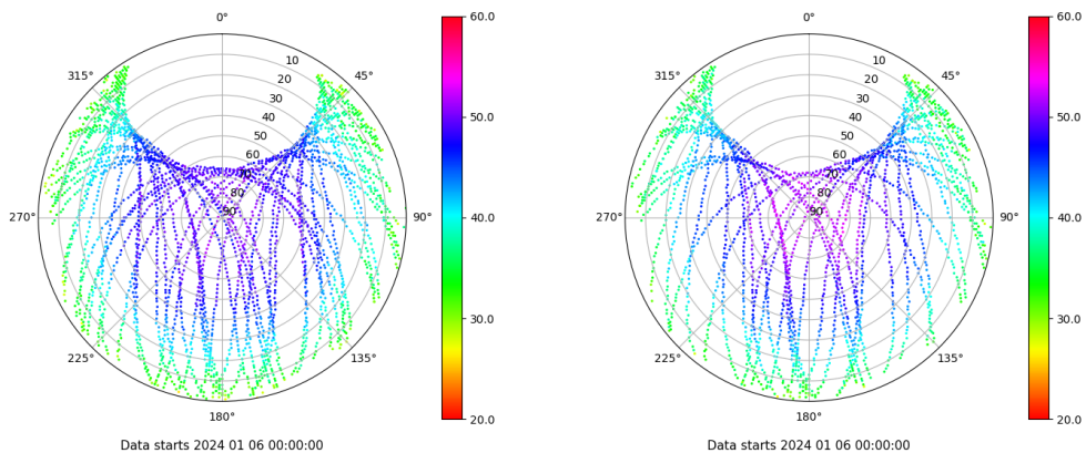
Skyplot for station SEV1. Signal to Noise S1C Data file SEV100ESP_R_2024006.xtr Skyplot for station SEV1. Signal to Noise S2X Data file SEV100ESP_R_2024006.xtr
