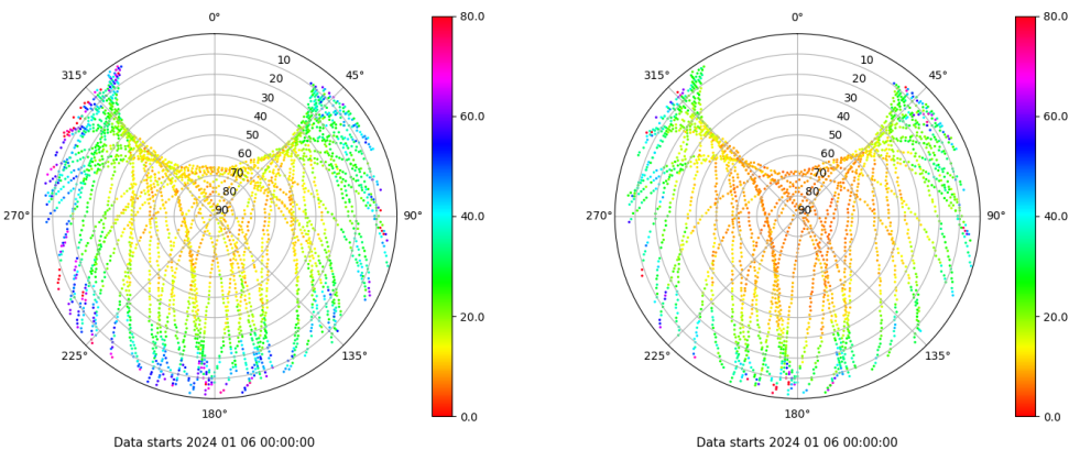
Skyplot for station SEV1. Parameter M1C Data file SEV100ESP_R_2024006.xtr Skyplot for station SEV1. Parameter M2X Data file SEV100ESP_R_2024006.xtr
