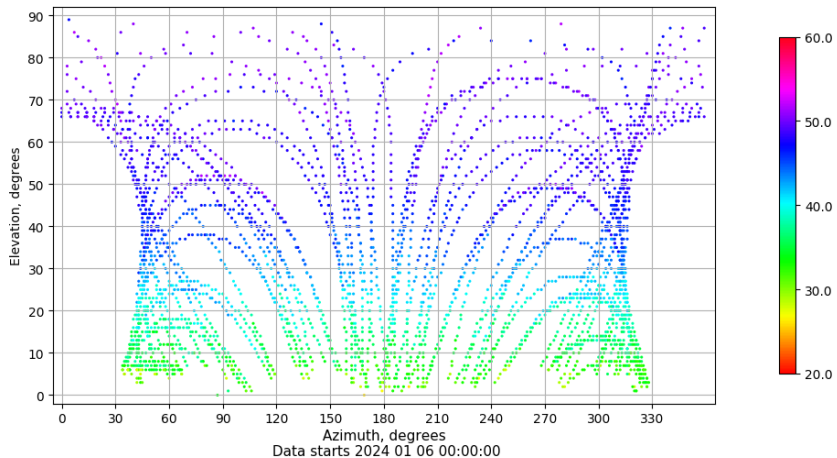
Azimuth-elevation plot for station SEV1. Signal to Noise S1C Data file SEV100ESP_R_2024006.xtr
