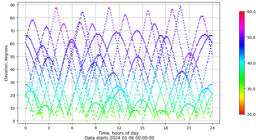
Time-elevation plot for station SEV1. Signal to Noise S1C Data file SEV100ESP_R_2024006.xtr
