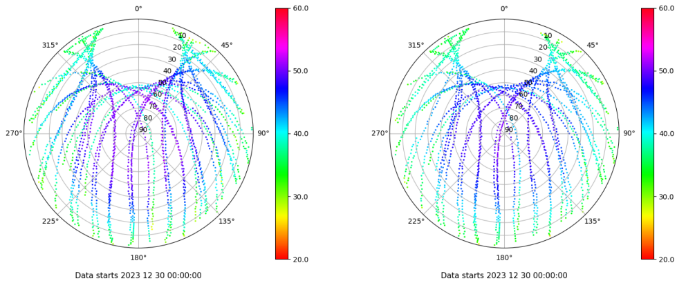
Skyplot for station SEV1. Signal to Noise S1C Data file SEV100ESP_R_2023364.xtr Skyplot for station SEV1. Signal to Noise S2C Data file SEV100ESP_R_2023364.xtr
