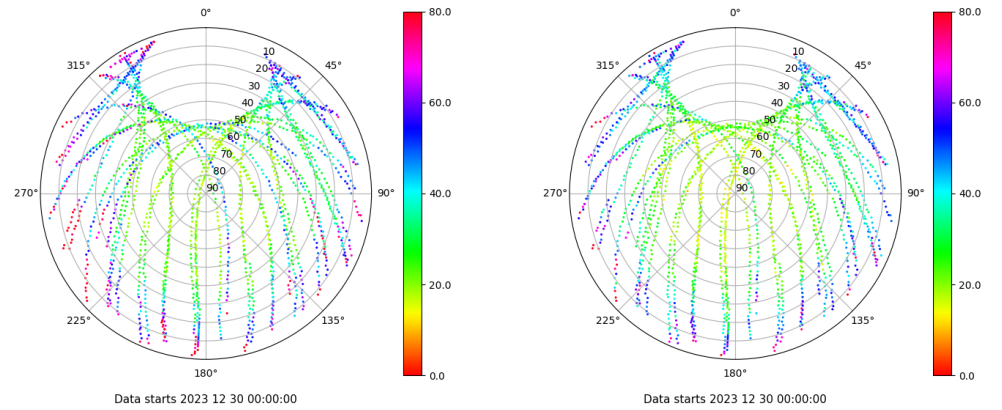
Skyplot for station SEV1. Parameter M1C Data file SEV100ESP_R_2023364.xtr Skyplot for station SEV1. Parameter M2C Data file SEV100ESP_R_2023364.xtr
