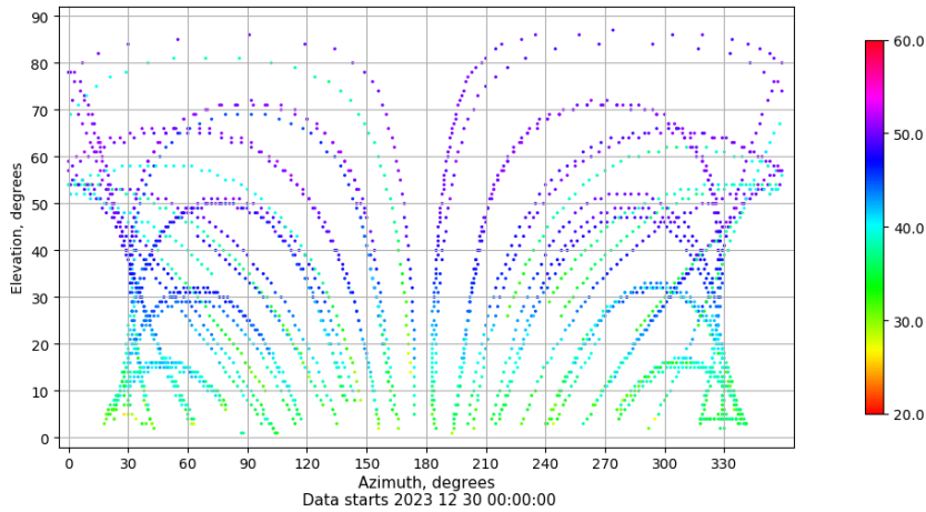
Azimuth-elevation plot for station SEV1. Signal to Noise S1C Data file SEV100ESP_R_2023364.xtr
