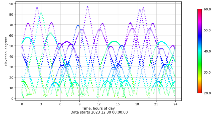
Time-elevation plot for station SEV1. Signal to Noise S1C Data file SEV100ESP_R_2023364.xtr
