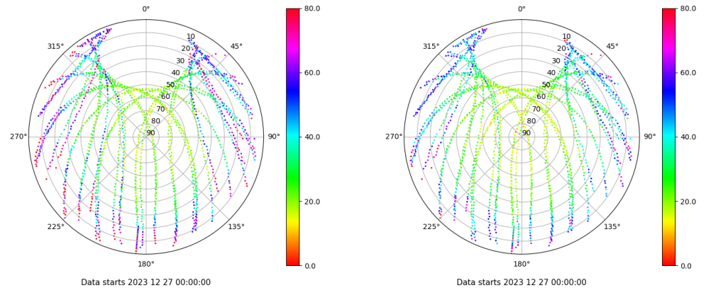
Skyplot for station SEV1. Parameter M1C Data file SEV100ESP_R_2023361.xtr Skyplot for station SEV1. Parameter M2C Data file SEV100ESP_R_2023361.xtr
