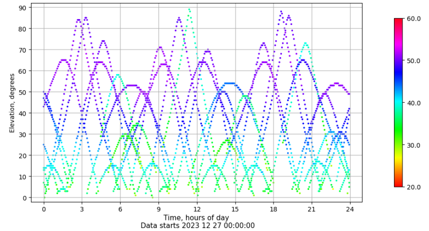
Time-elevation plot for station SEV1. Signal to Noise S1C Data file SEV100ESP_R_2023361.xtr
