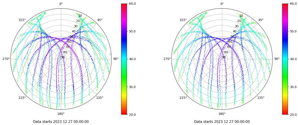
Skyplot for station SEV1. Signal to Noise S1C Data file SEV100ESP_R_2023361.xtr Skyplot for station SEV1. Signal to Noise S2C Data file SEV100ESP_R_2023361.xtr
