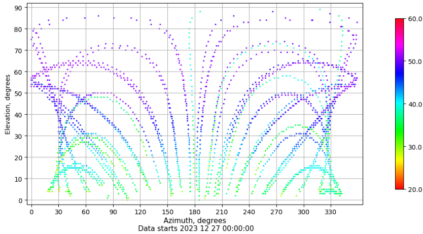
Azimuth-elevation plot for station SEV1. Signal to Noise S1C Data file SEV100ESP_R_2023361.xtr
