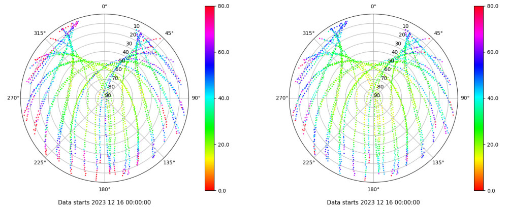
Skyplot for station SEV1. Parameter M1C Data file SEV100ESP_R_2023350.xtr Skyplot for station SEV1. Parameter M2C Data file SEV100ESP_R_2023350.xtr
