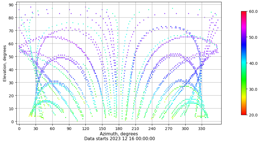
Azimuth-elevation plot for station SEV1. Signal to Noise S1C Data file SEV100ESP_R_2023350.xtr
