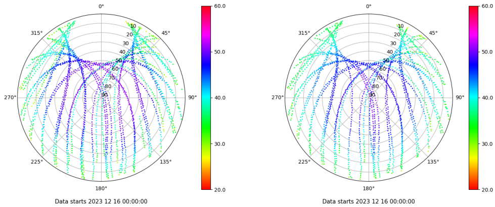
Skyplot for station SEV1. Signal to Noise S1C Data file SEV100ESP_R_2023350.xtr Skyplot for station SEV1. Signal to Noise S2C Data file SEV100ESP_R_2023350.xtr
