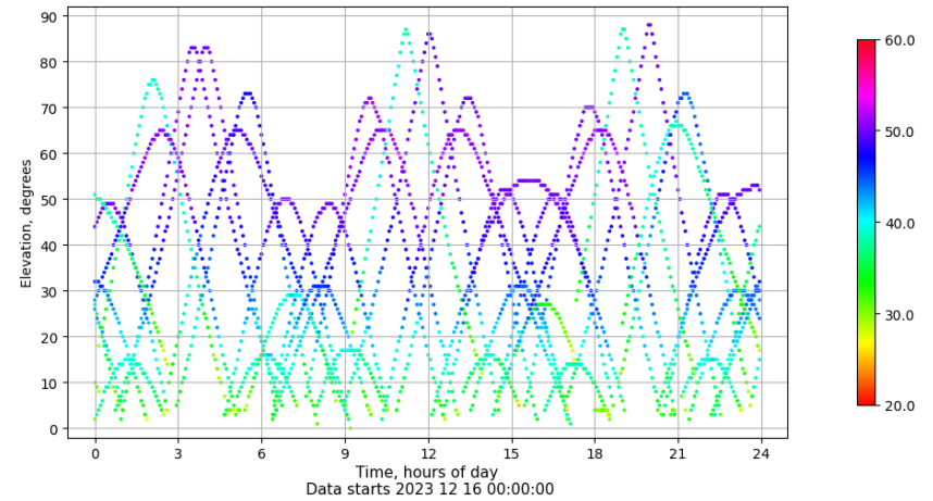
Time-elevation plot for station SEV1. Signal to Noise S1C Data file SEV100ESP_R_2023350.xtr
