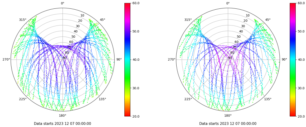
Skyplot for station SEV1. Signal to Noise S1C Data file SEV100ESP_R_2023341.xtr Skyplot for station SEV1. Signal to Noise S2X Data file SEV100ESP_R_2023341.xtr
