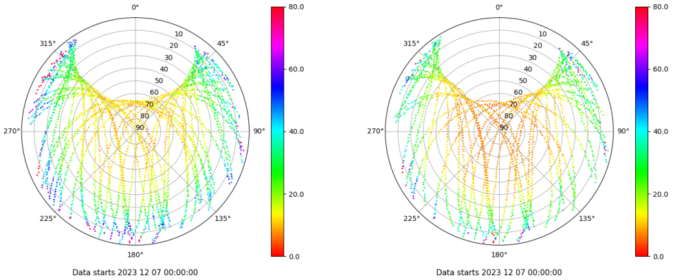
Skyplot for station SEV1. Parameter M1C Data file SEV100ESP_R_2023341.xtr Skyplot for station SEV1. Parameter M2X Data file SEV100ESP_R_2023341.xtr
