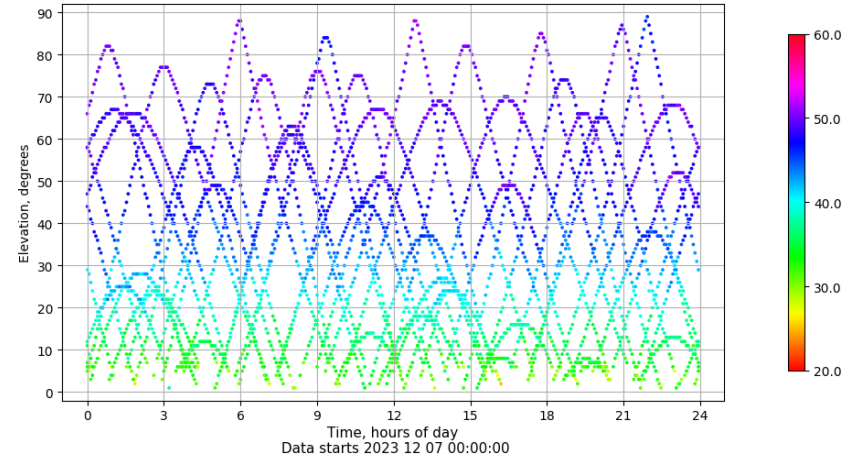
Time-elevation plot for station SEV1. Signal to Noise S1C Data file SEV100ESP_R_2023341.xtr
