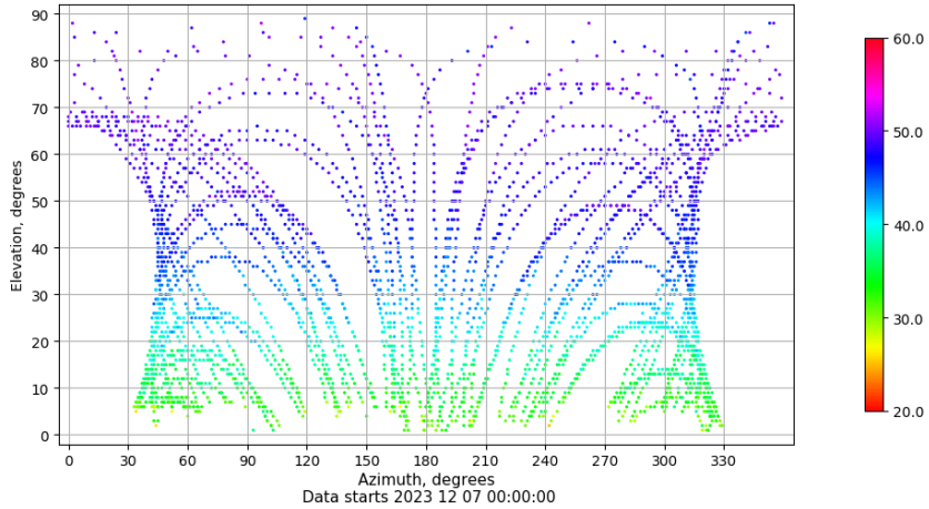
Azimuth-elevation plot for station SEV1. Signal to Noise S1C Data file SEV100ESP_R_2023341.xtr
