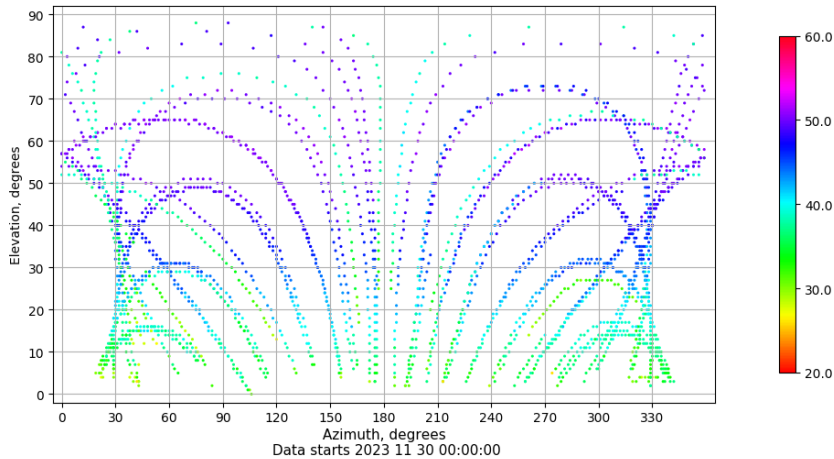
Azimuth-elevation plot for station SEV1. Signal to Noise S1C Data file SEV100ESP_R_2023334.xtr
