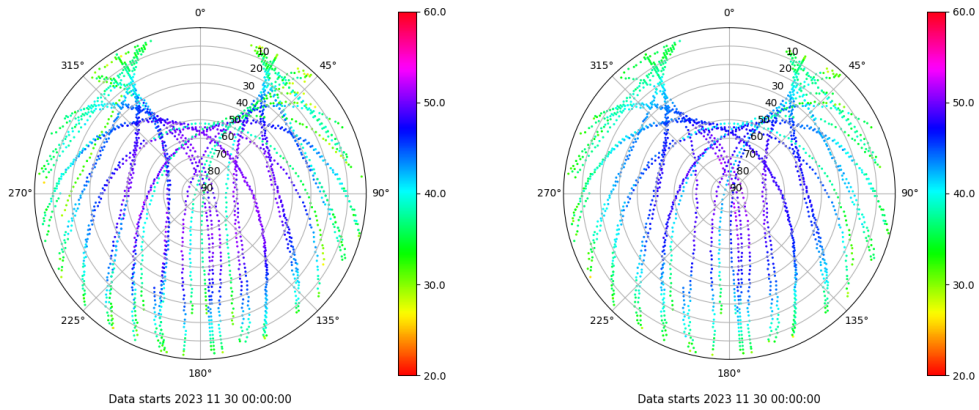
Skyplot for station SEV1. Signal to Noise S1C Data file SEV100ESP_R_2023334.xtr Skyplot for station SEV1. Signal to Noise S2C Data file SEV100ESP_R_2023334.xtr
