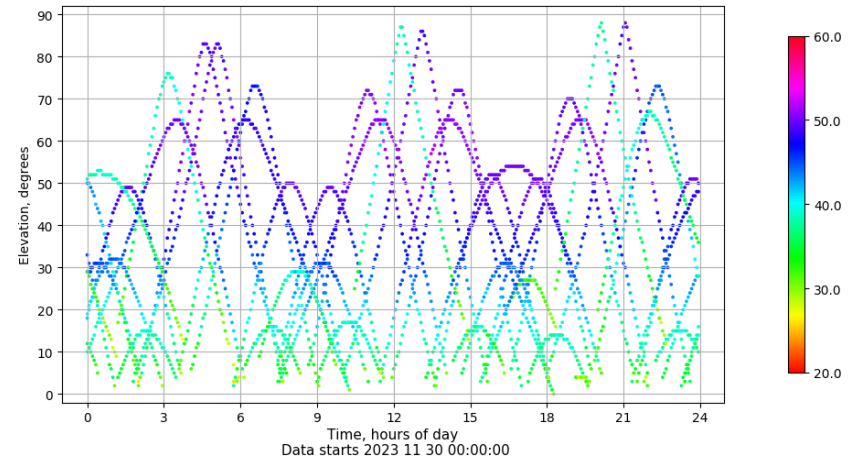
Time-elevation plot for station SEV1. Signal to Noise S1C Data file SEV100ESP_R_2023334.xtr
