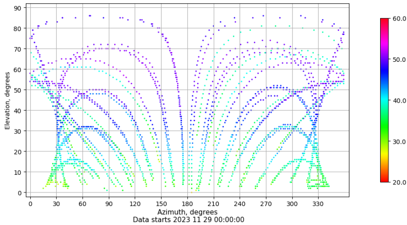
Azimuth-elevation plot for station SEV1. Signal to Noise S1C Data file SEV100ESP_R_2023333.xtr
