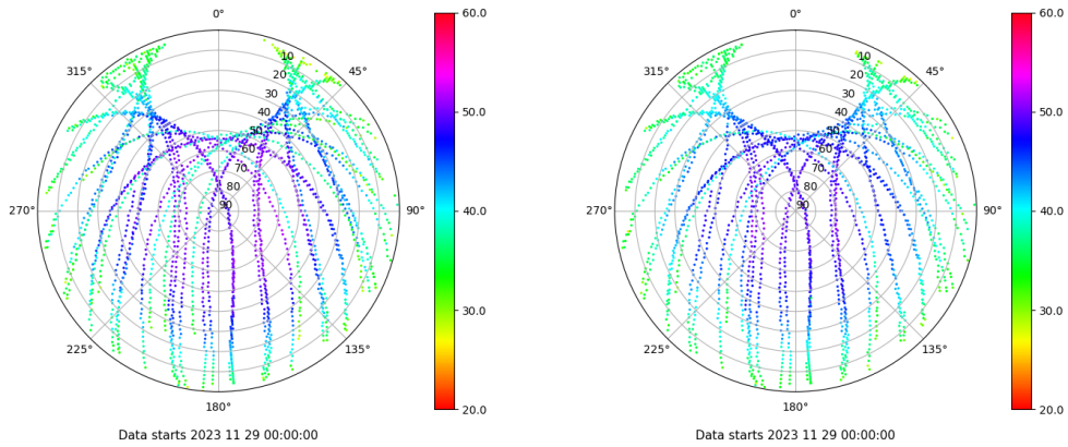
Skyplot for station SEV1. Signal to Noise S1C Data file SEV100ESP_R_2023333.xtr Skyplot for station SEV1. Signal to Noise S2C Data file SEV100ESP_R_2023333.xtr
