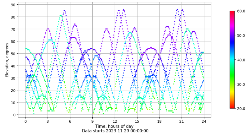
Time-elevation plot for station SEV1. Signal to Noise S1C Data file SEV100ESP_R_2023333.xtr
