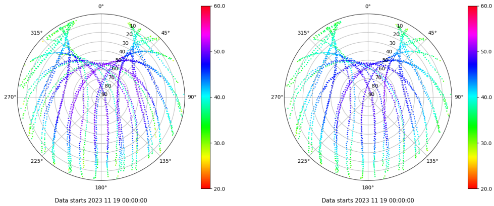
Skyplot for station SEV1. Signal to Noise S1C Data file SEV100ESP_R_2023323.xtr Skyplot for station SEV1. Signal to Noise S2C Data file SEV100ESP_R_2023323.xtr
