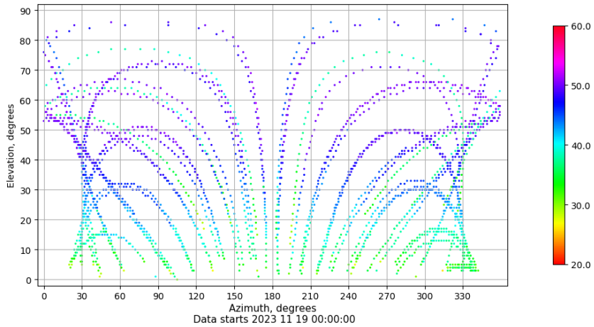
Azimuth-elevation plot for station SEV1. Signal to Noise S1C Data file SEV100ESP_R_2023323.xtr
