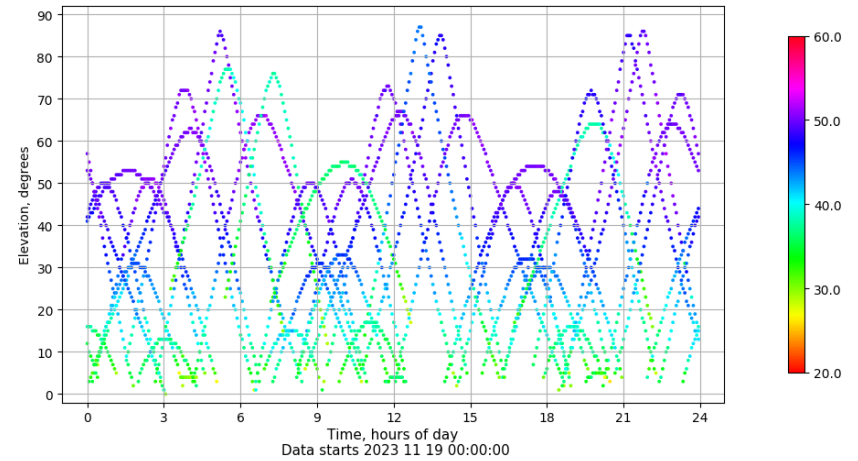
Time-elevation plot for station SEV1. Signal to Noise S1C Data file SEV100ESP_R_2023323.xtr
