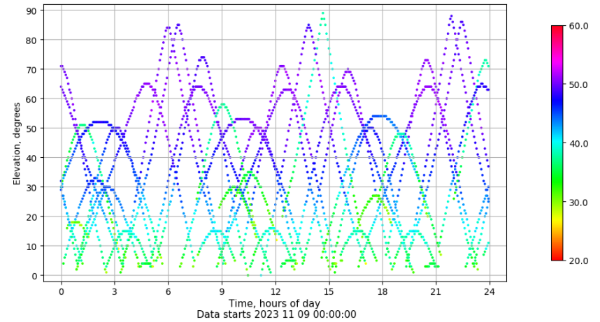
Time-elevation plot for station SEV1. Signal to Noise S1C Data file SEV100ESP_R_2023313.xtr
