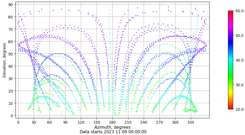
Azimuth-elevation plot for station SEV1. Signal to Noise S1C Data file SEV100ESP_R_2023313.xtr
