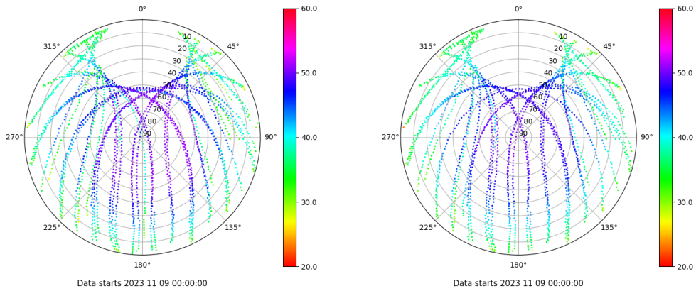
Skyplot for station SEV1. Signal to Noise S1C Data file SEV100ESP_R_2023313.xtr Skyplot for station SEV1. Signal to Noise S2C Data file SEV100ESP_R_2023313.xtr
