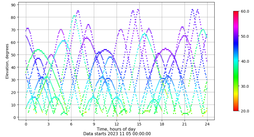
Time-elevation plot for station SEV1. Signal to Noise S1C Data file SEV100ESP_R_2023309.xtr
