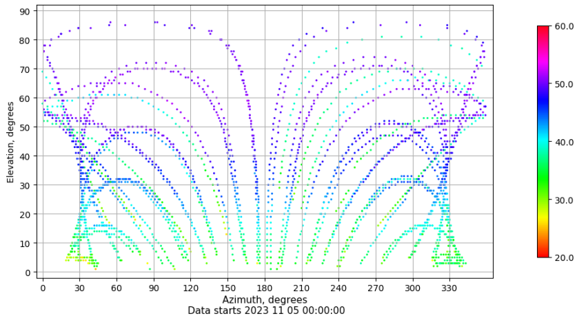
Azimuth-elevation plot for station SEV1. Signal to Noise S1C Data file SEV100ESP_R_2023309.xtr
