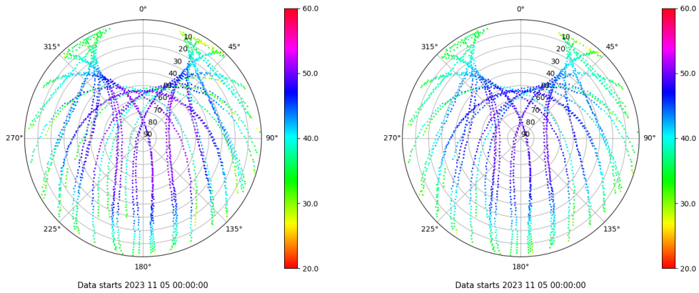
Skyplot for station SEV1. Signal to Noise S1C Data file SEV100ESP_R_2023309.xtr Skyplot for station SEV1. Signal to Noise S2C Data file SEV100ESP_R_2023309.xtr
